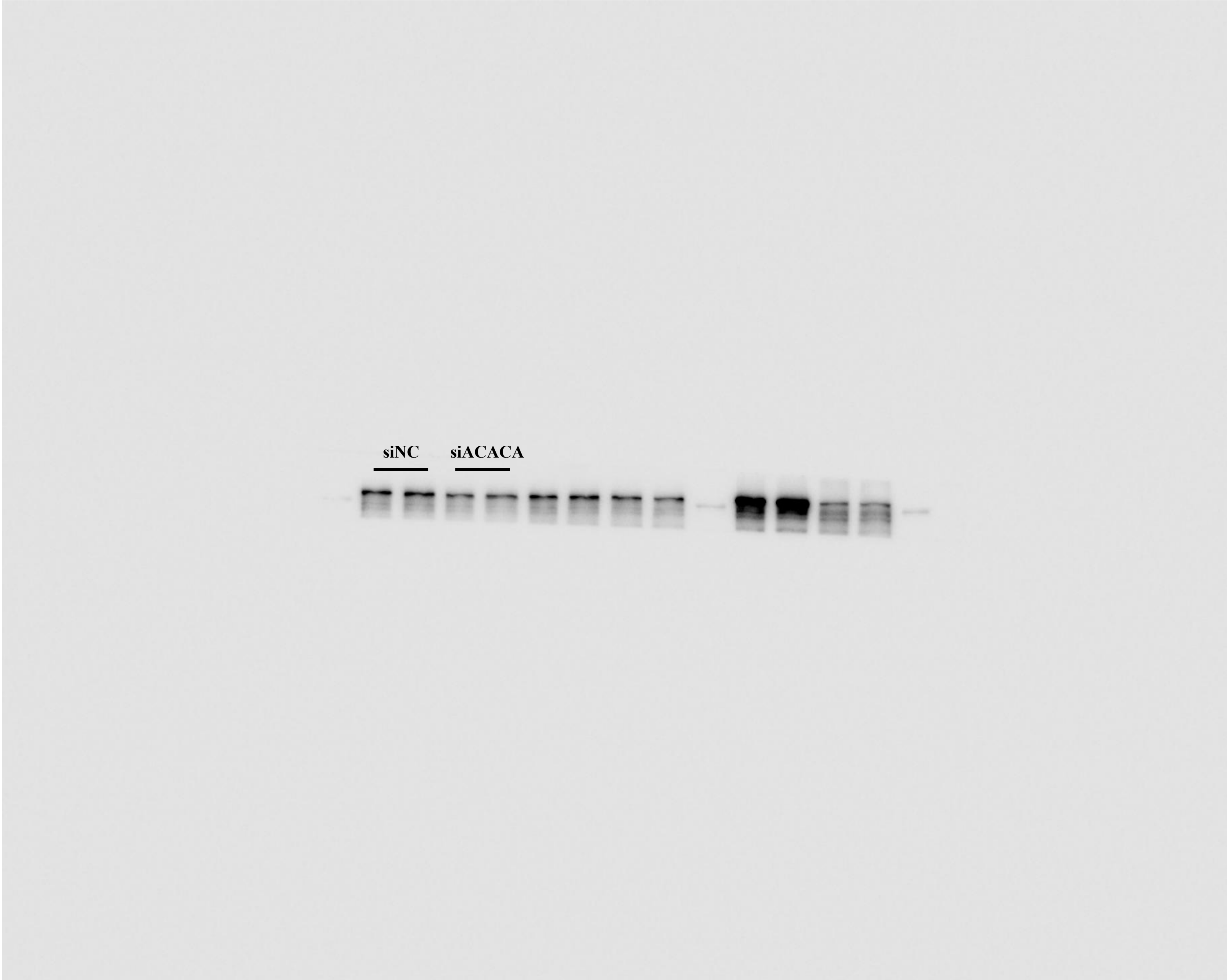
Figure 7D ACACA
