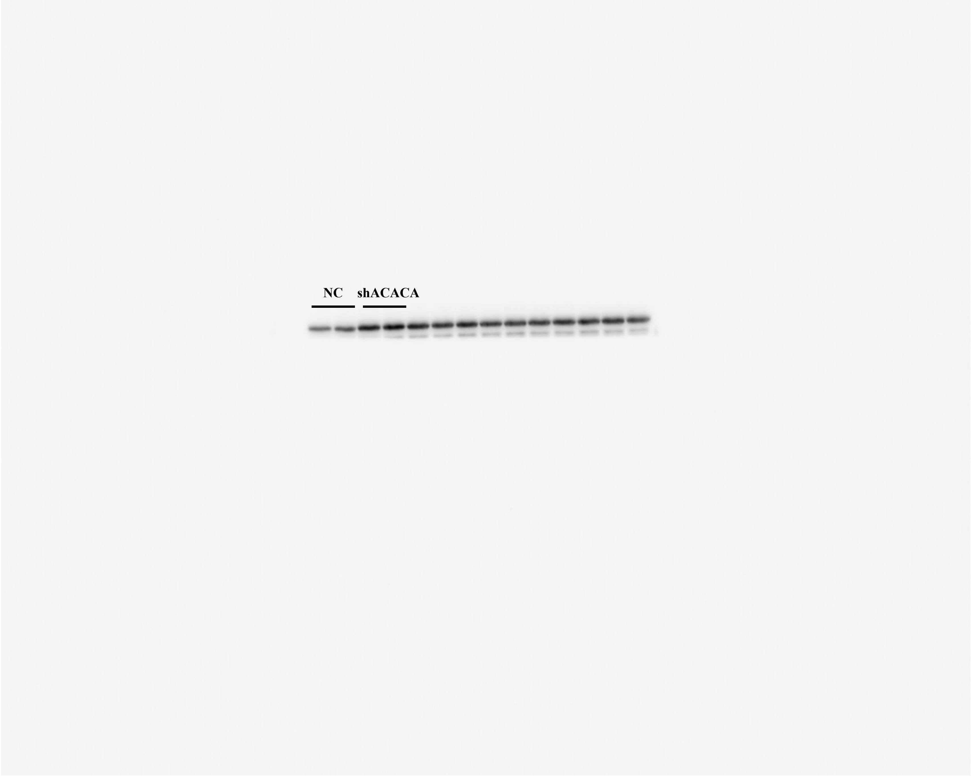
Figure 7A pP65
