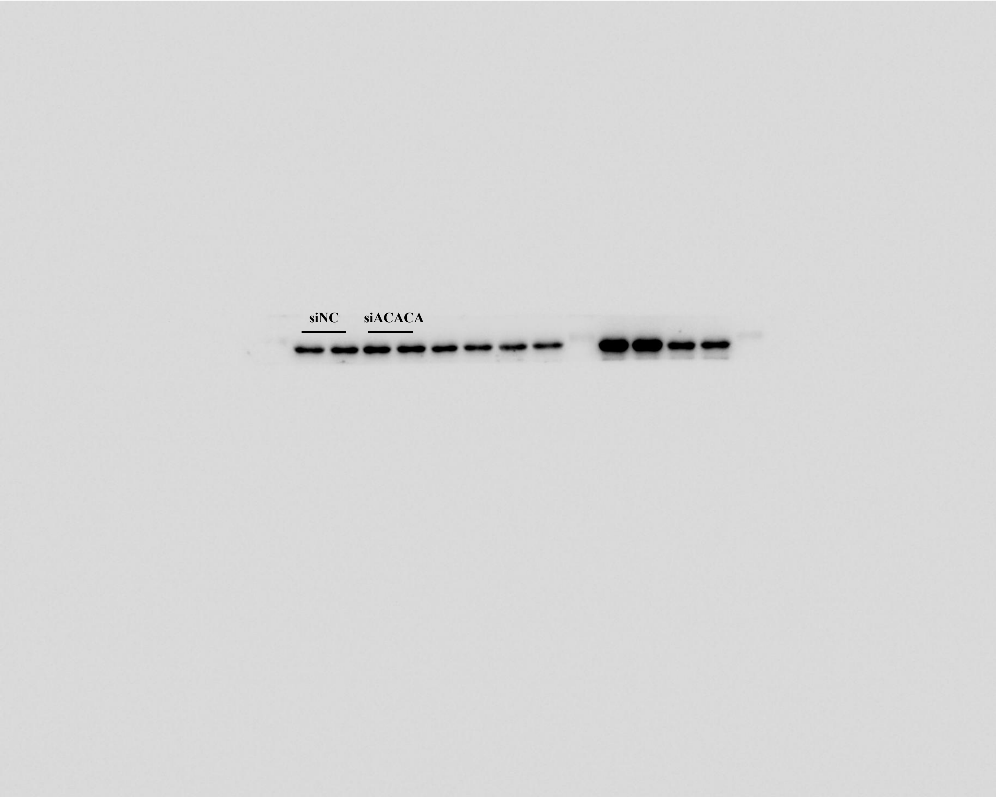
Figure 7D pP65
