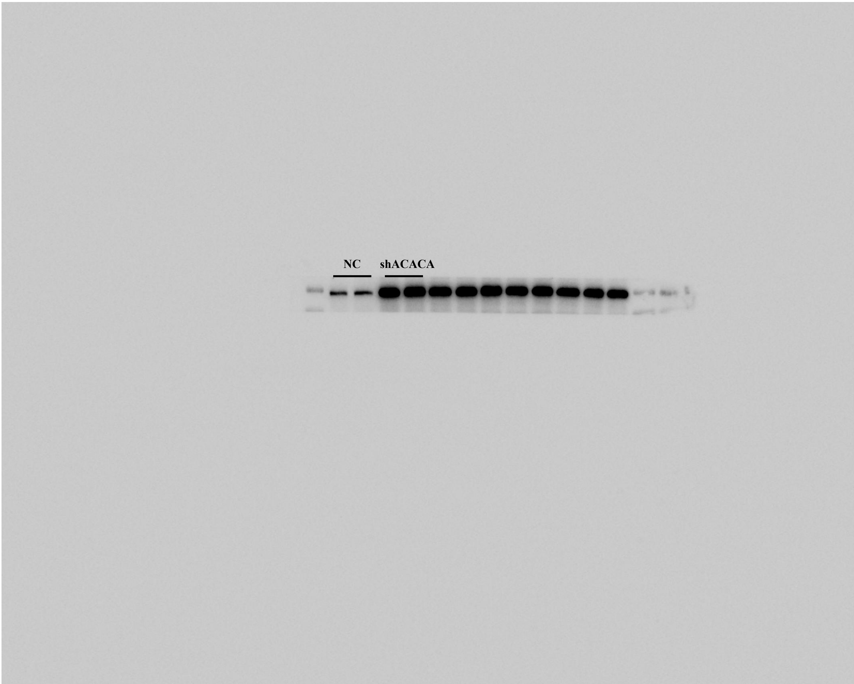
Figure 7A IKKβ
