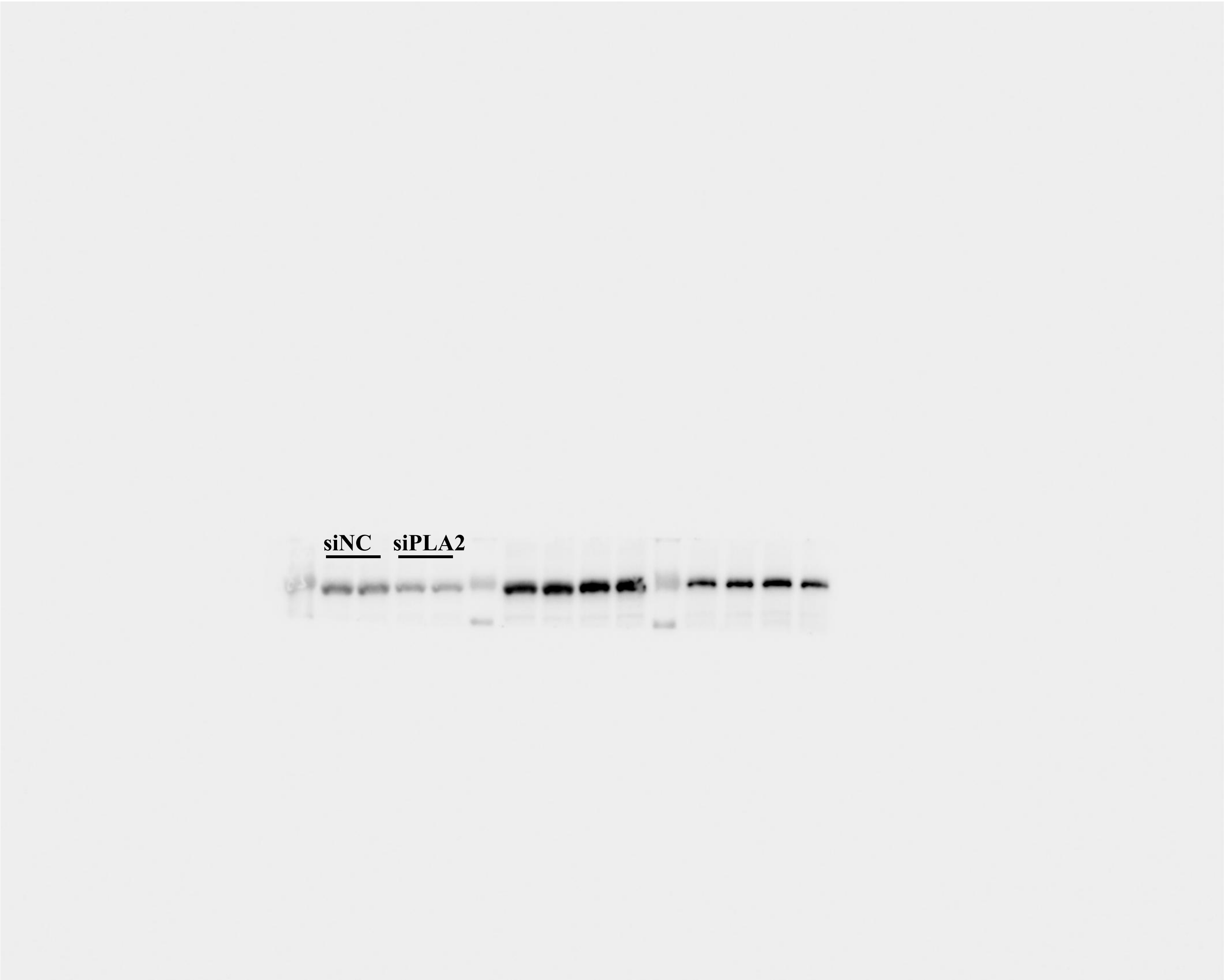
Figure 7N pP65
