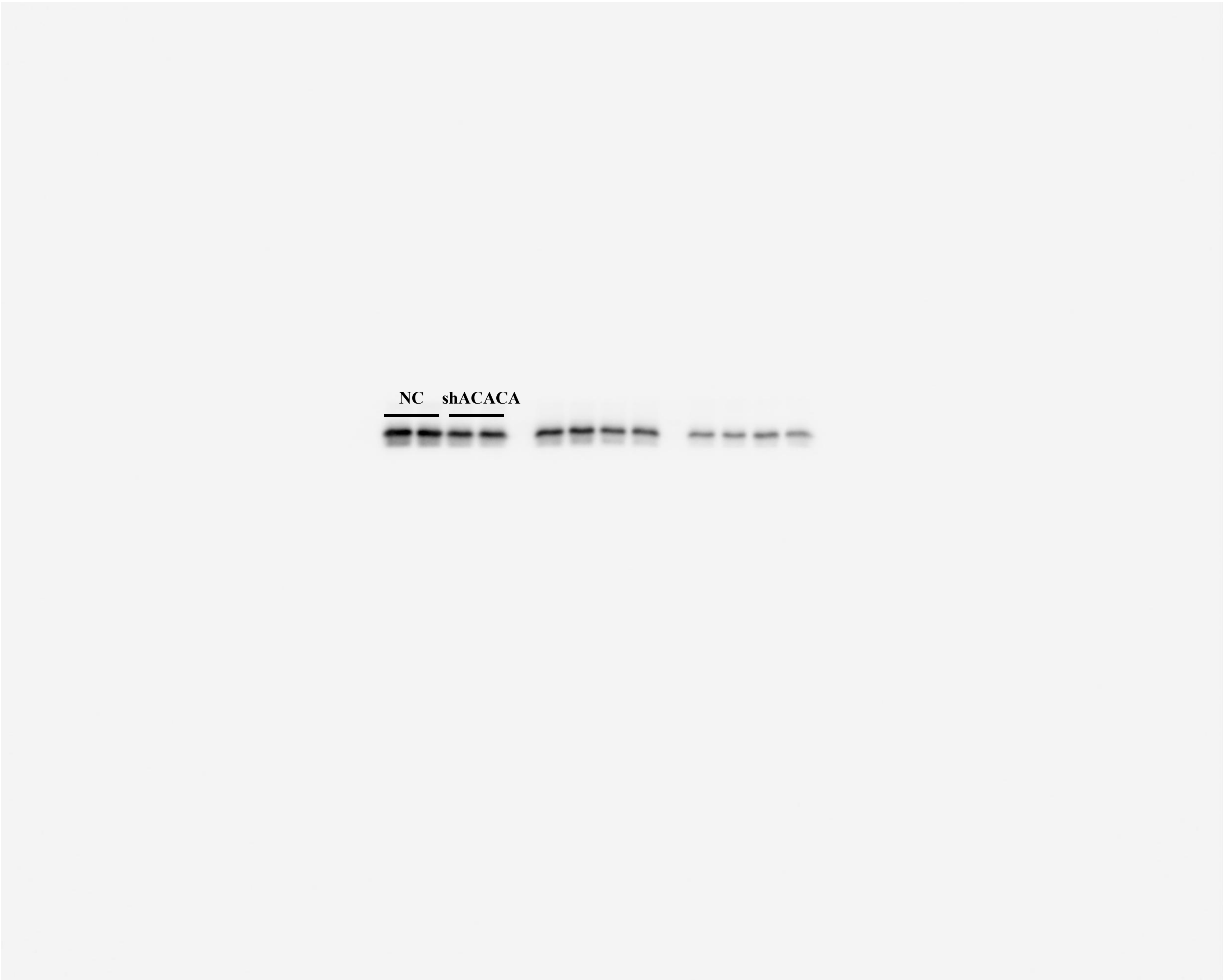
Figure 7A IκBa
