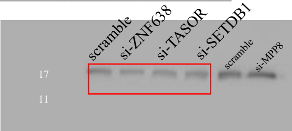
Original images to Figure 5. Original image to Figure 5B H3, ZNF638, MPP8, H3K9me3, H3K4me3 and H3K27ac.
