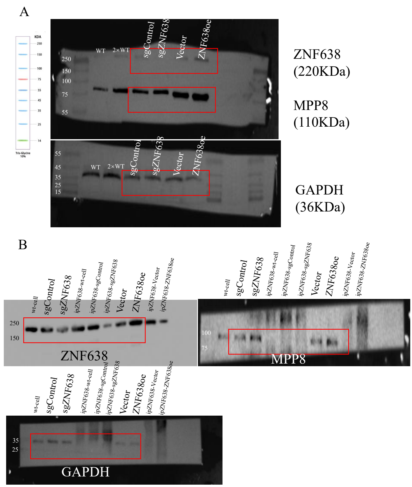
Original images to Supplement Figure 2. (A). Original image to Supplement Figure 2C, D-ZNF638, MPP8 and GAPDH. (B). Original images from repetitive experiments to Figure 2C, D-ZNF638, MPP8 and GAPDH.
