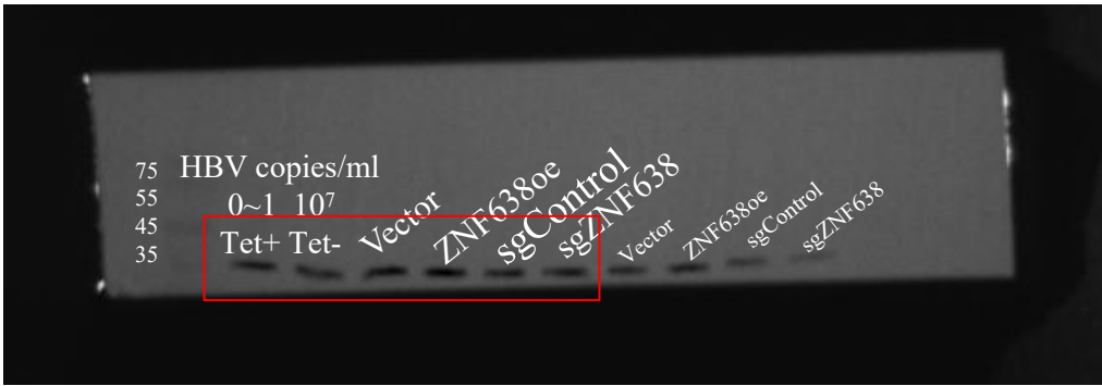
Original images to Figure 1. (A) Original image to Figure 1C-E-ZNF638 and GAPDH.(B) Original image to Figure 1H-J-ZNF638 and GAPDH.
