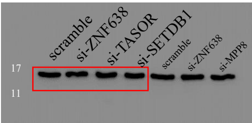
Original images to Figure 5. Original image to Figure 5B H3, ZNF638, MPP8, H3K9me3, H3K4me3 and H3K27ac.
