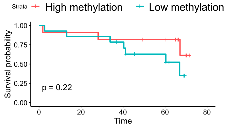
C) TCGA-COAD: Global \beta methylation in tumor tissue
