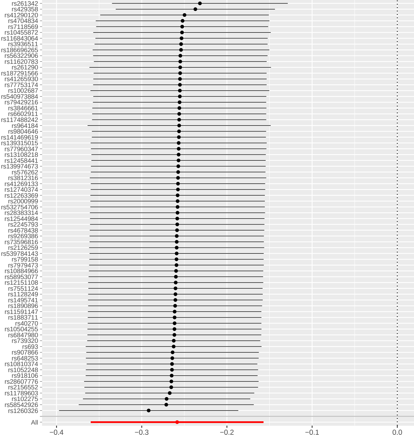
MR leave-one-out sensitivity analysis for ' || id:met-d-SFA' on 'Early age-related macular degeneration || id:ebi-a-GCST010723'
