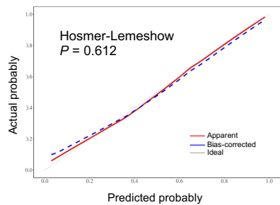
Figure S1. Calibration Curve and Decision Curve Analysis of the Exo-miRNAs Panel.
