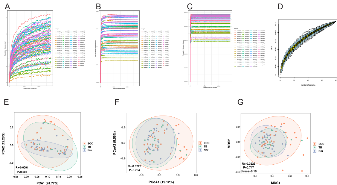
Fig S1 Quality of microbial sequencing data and its \beta -diversity. A, B, C illustrate the Rarefaction Curve plots for Chao1, Shannon, and Simpson indices, respectively. D Species Accumulation Curves. E principal component analysis (PCA) among three groups. F principal coordinate analysis (PCoA) among three groups. G non-metric multidimensional scaling analysis (NMDS) among three groups. P values and R values were calculated by the ANOSIM test.
