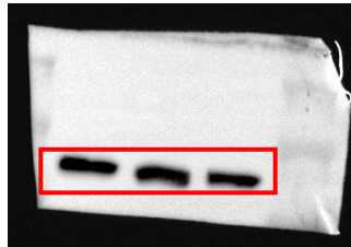
FN1 285KDa
