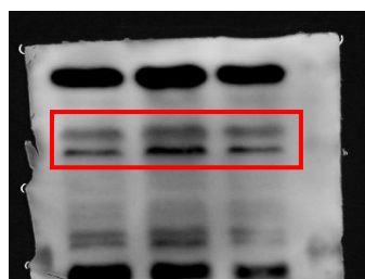
P-c-JNK 46/54KDa
