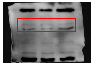
P-c-JNK 46/54KDa
