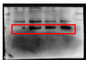
FN1 285KDa
