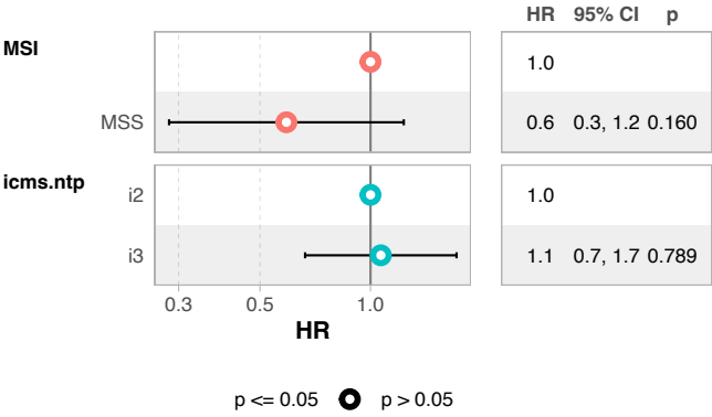
Figure S6. Forest plot representation of multivariable models including MSI status and icMS class.
