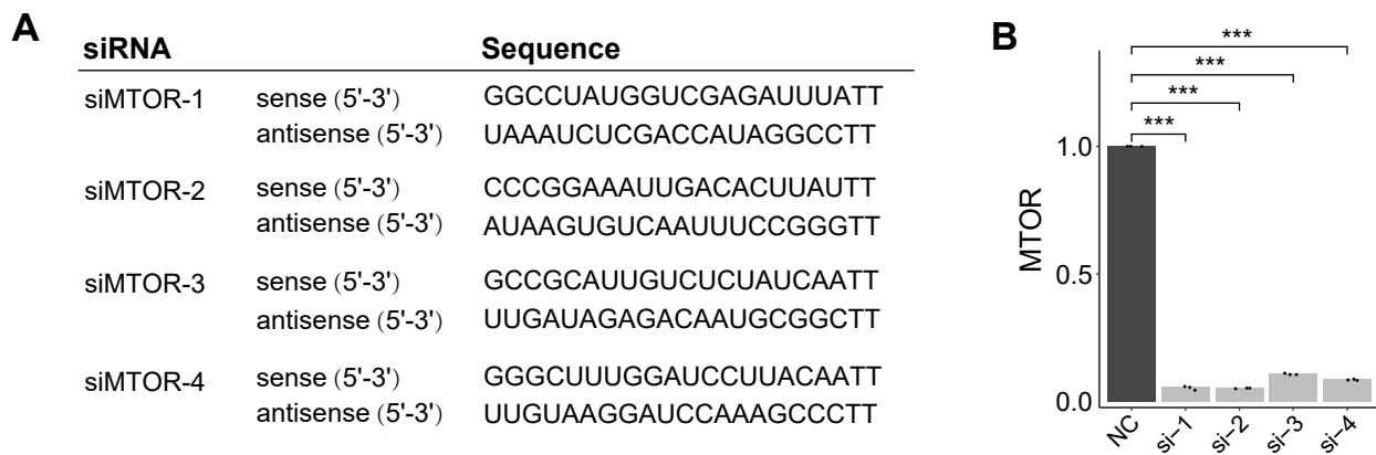
Figure S6. Knockdown efficiency of MTOR -targeting siRNAs.
