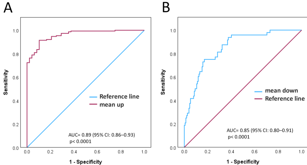
Figure S2. Sensitivity analysis of circulating miRNA panels in the prospective MENA cohort. (A) ROC curve of the mean expression score for the 8 upregulated miRNAs ( n = 152 breast cancer, n = 48 prospectively collected controls), demonstrating robust discrimination (AUC = 0.89, 95% CI: 0.86–0.93, p < 0.0001 ). (B) ROC curve of the mean expression score for the 11 downregulated miRNAs, showing consistent discrimination between breast cancer patients and prospective controls (AUC = 0.85, 95% CI: 0.80–0.91, p < 0.0001 ).
