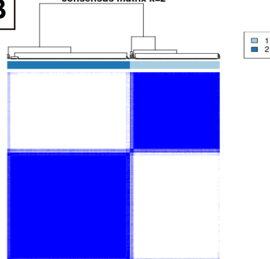
consensus matrix k=2
