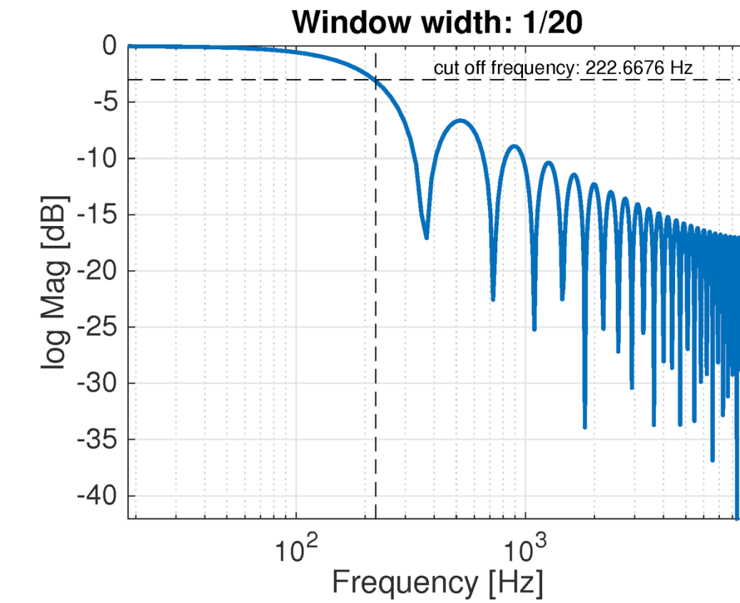
FIG S4: Magnitude Responses of the temporal filtering
