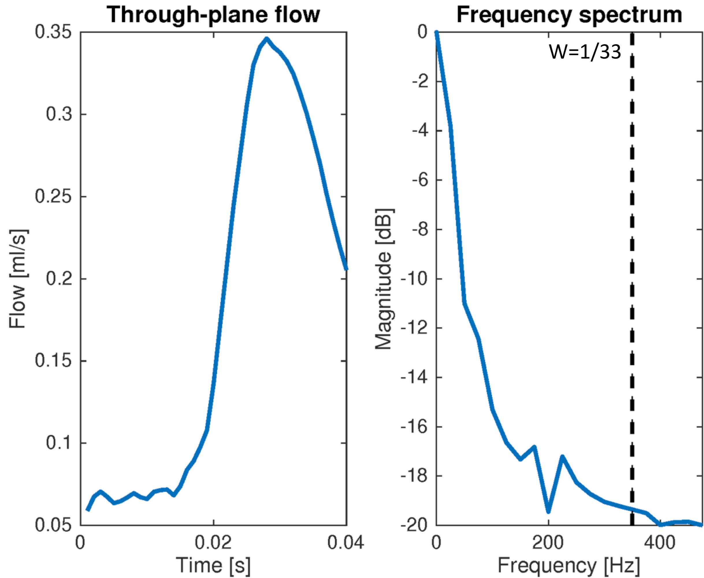
FIG S5: Frequency analysis of a high-resolution (1 ms) flow measurement
