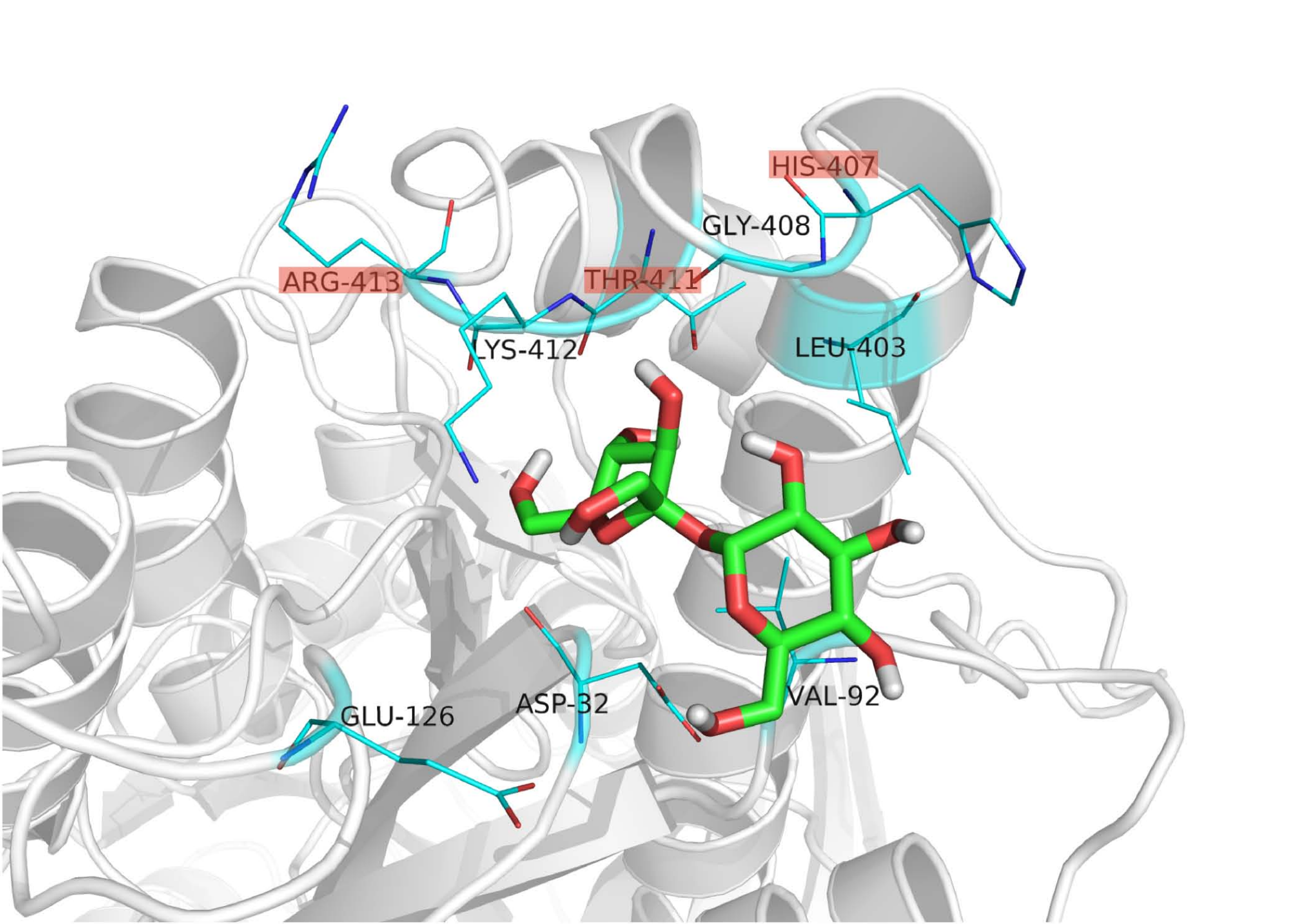
sucrose
