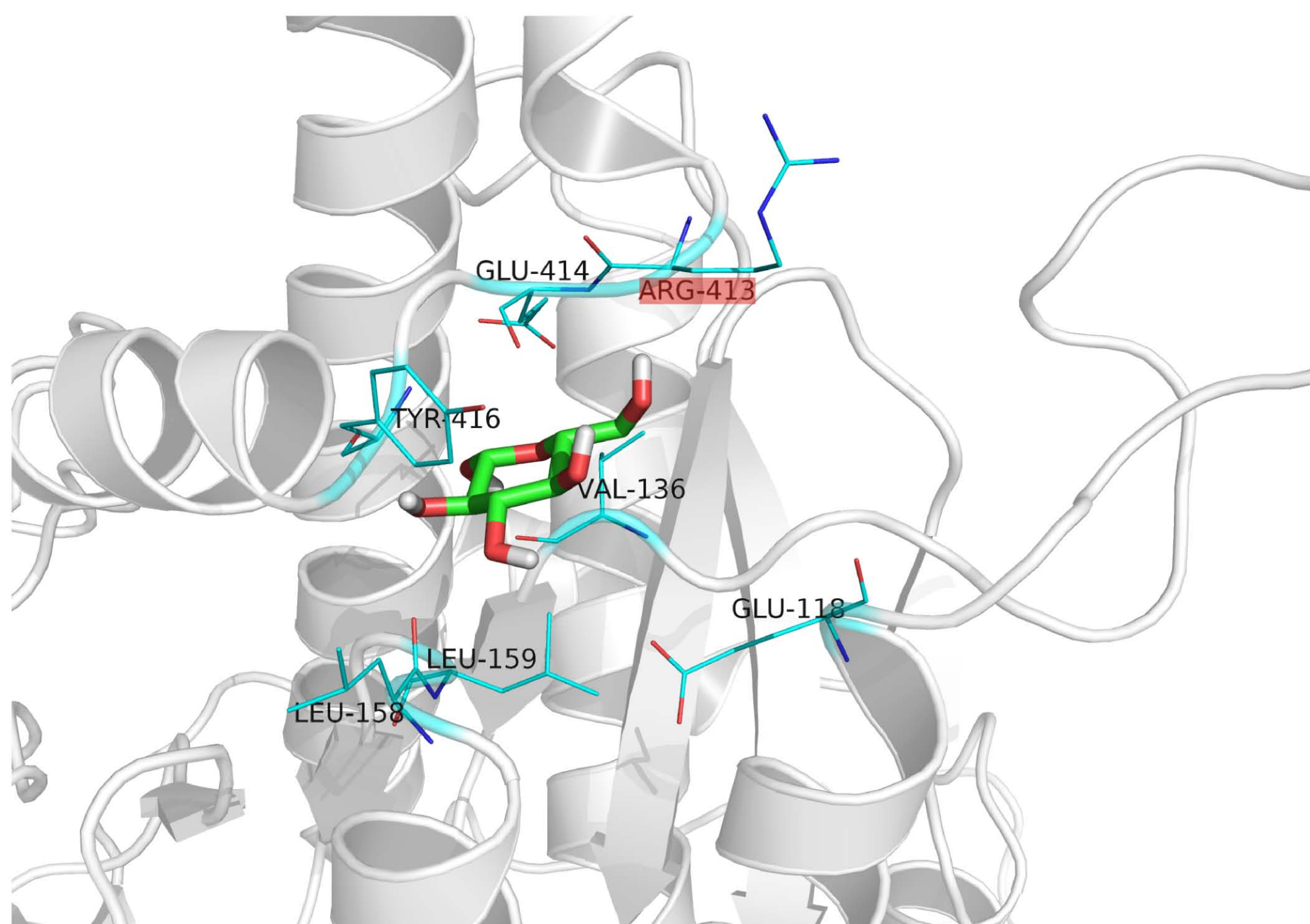
D-glucose
