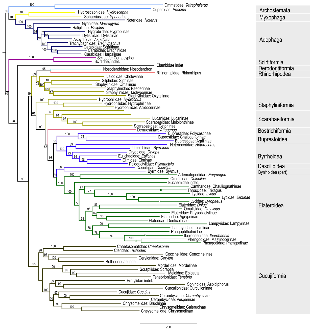
Supplementary Figure S2. Maximum likelihood tree for 83 species of beetles recovered from 15 mitochondrial genes.
