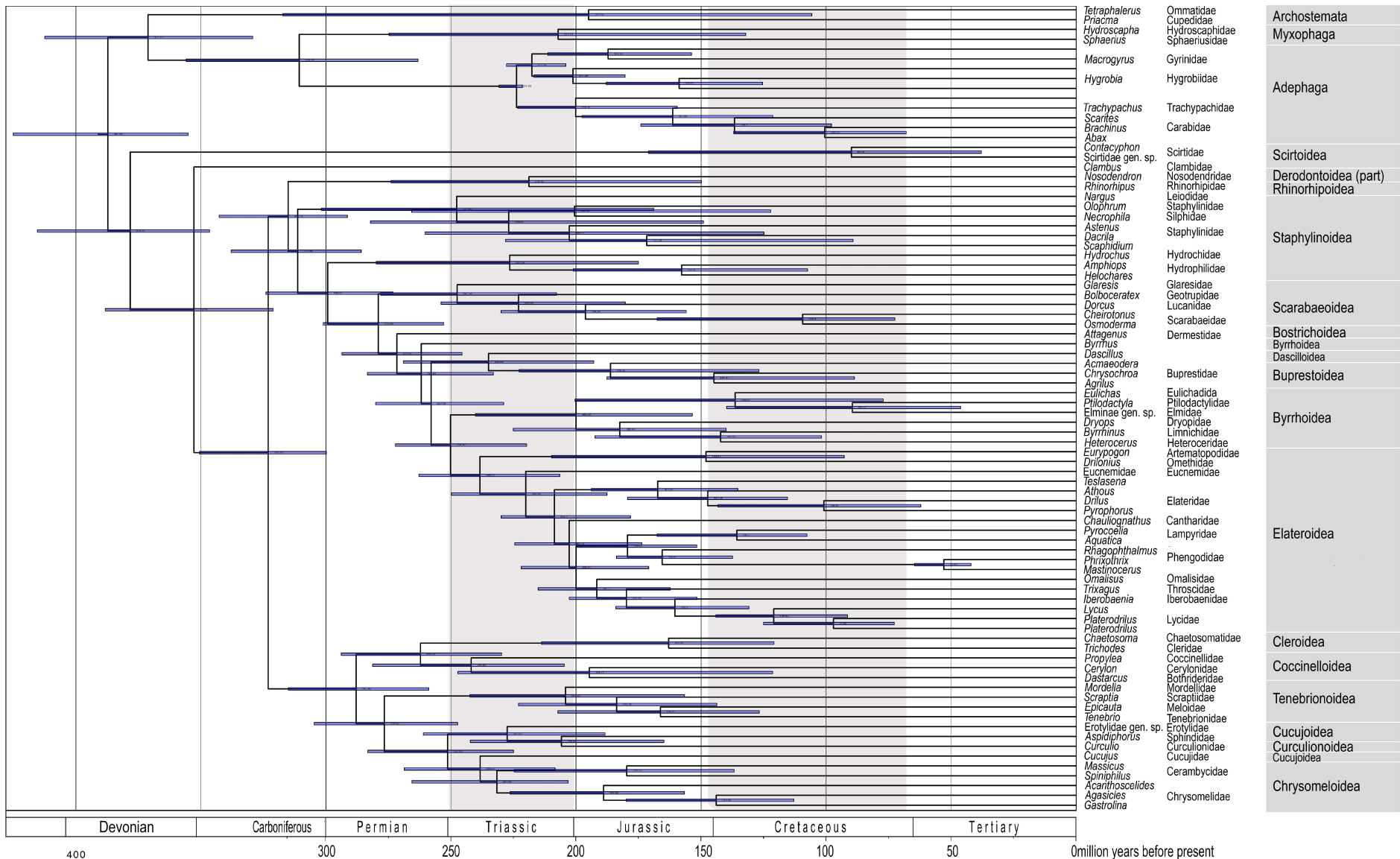
Supplementary Figure S10. Dated phylogenetic tree of insect relationships inferred from the Bayesian analysis of mitogenomic dataset using the Bayesian topology.
