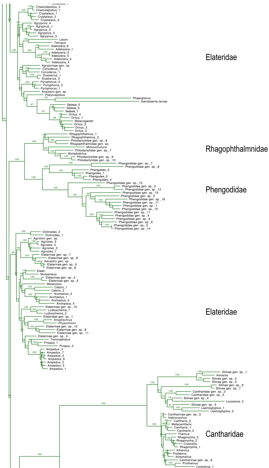
Supplementary Figure 1. Continued (Part 3).
