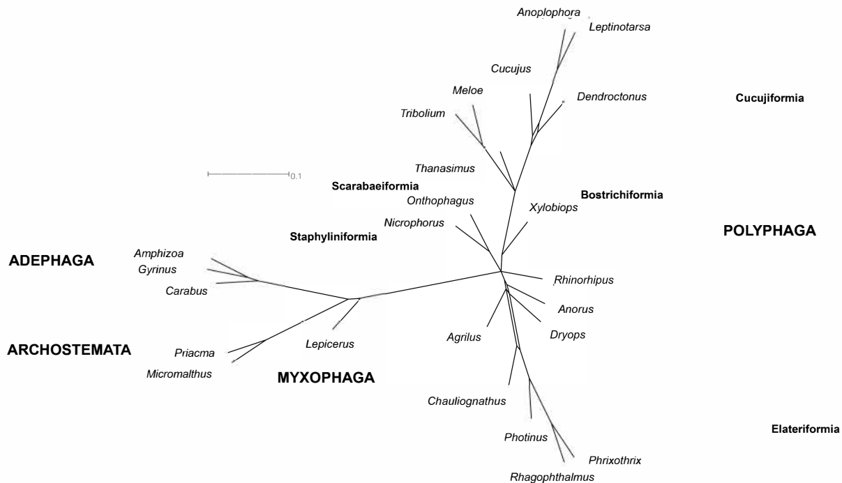
Supplementary Figure S8. Tree network obtained from the separate maximum likelihood analyses of 968 orthologs.
