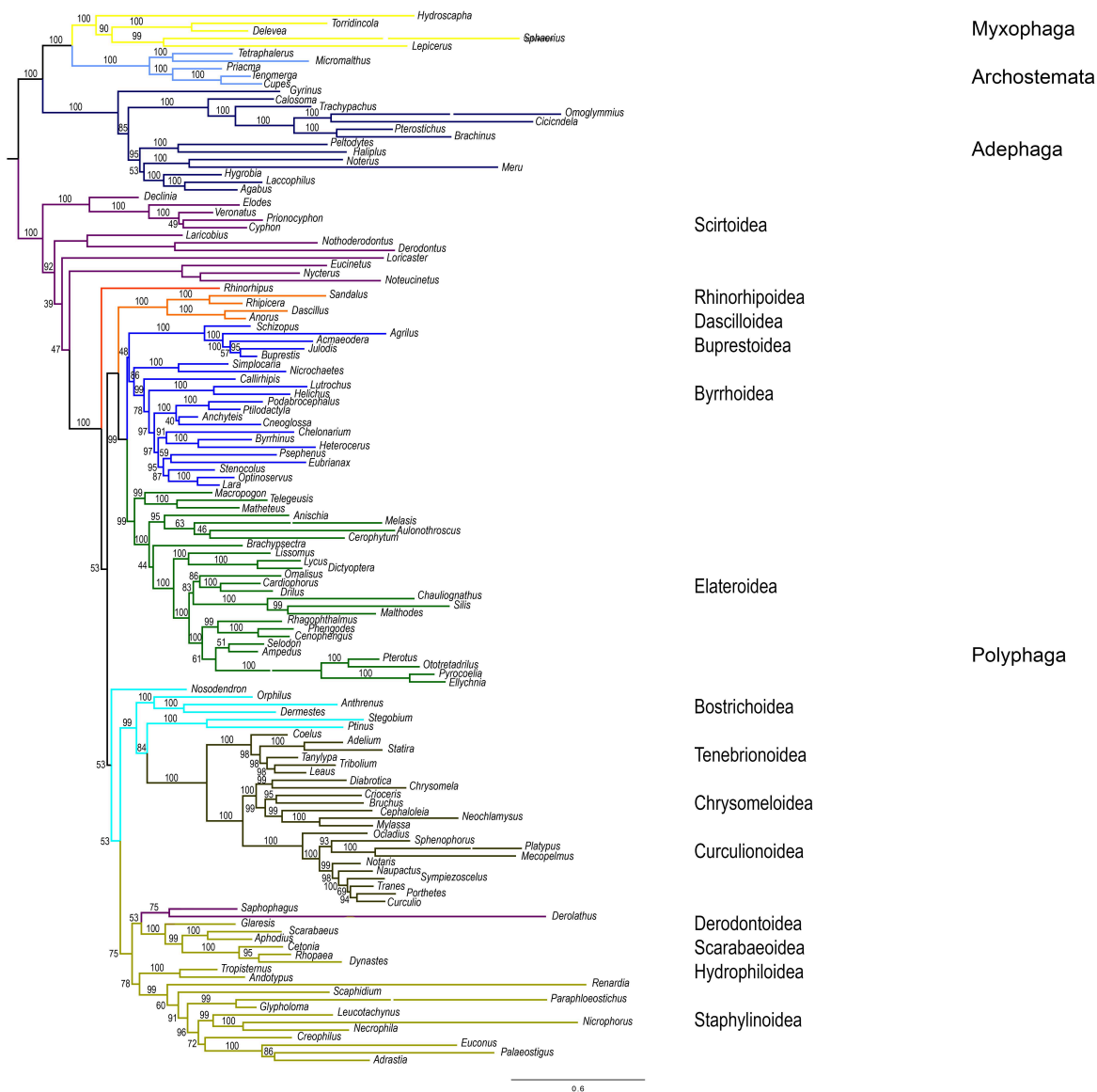
Supplementary Figure 4. Bayesian tree for 139 species of beetles recovered from the 18S rRNA, 28S rRNA and six protein coding nuclear genes.
