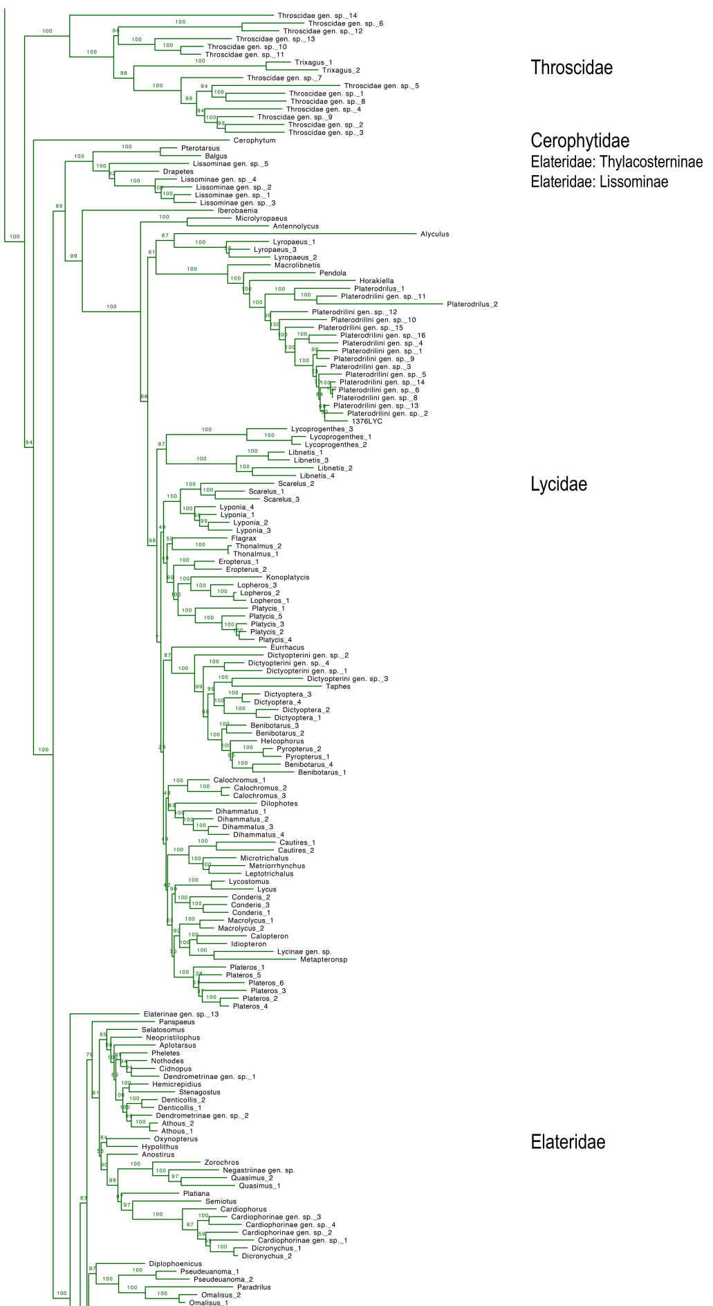
Supplementary Figure 1. Continued (Part 2).
