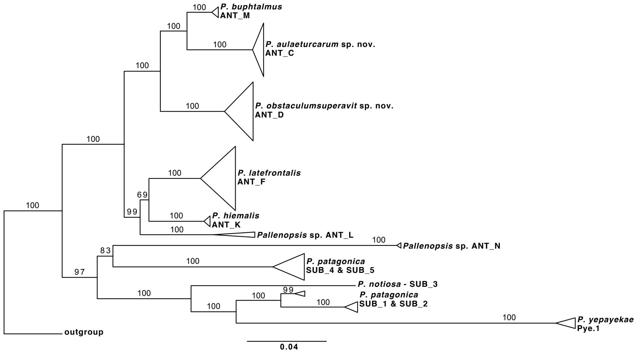
Additional file 2: Phylogenetic SNP tree of the Pallenopsis patagonica species complex. Maximum-Likelihood tree based on aligned SNP data of all Pallenopsis samples. Bootstrap values are given next to the respective branches.
