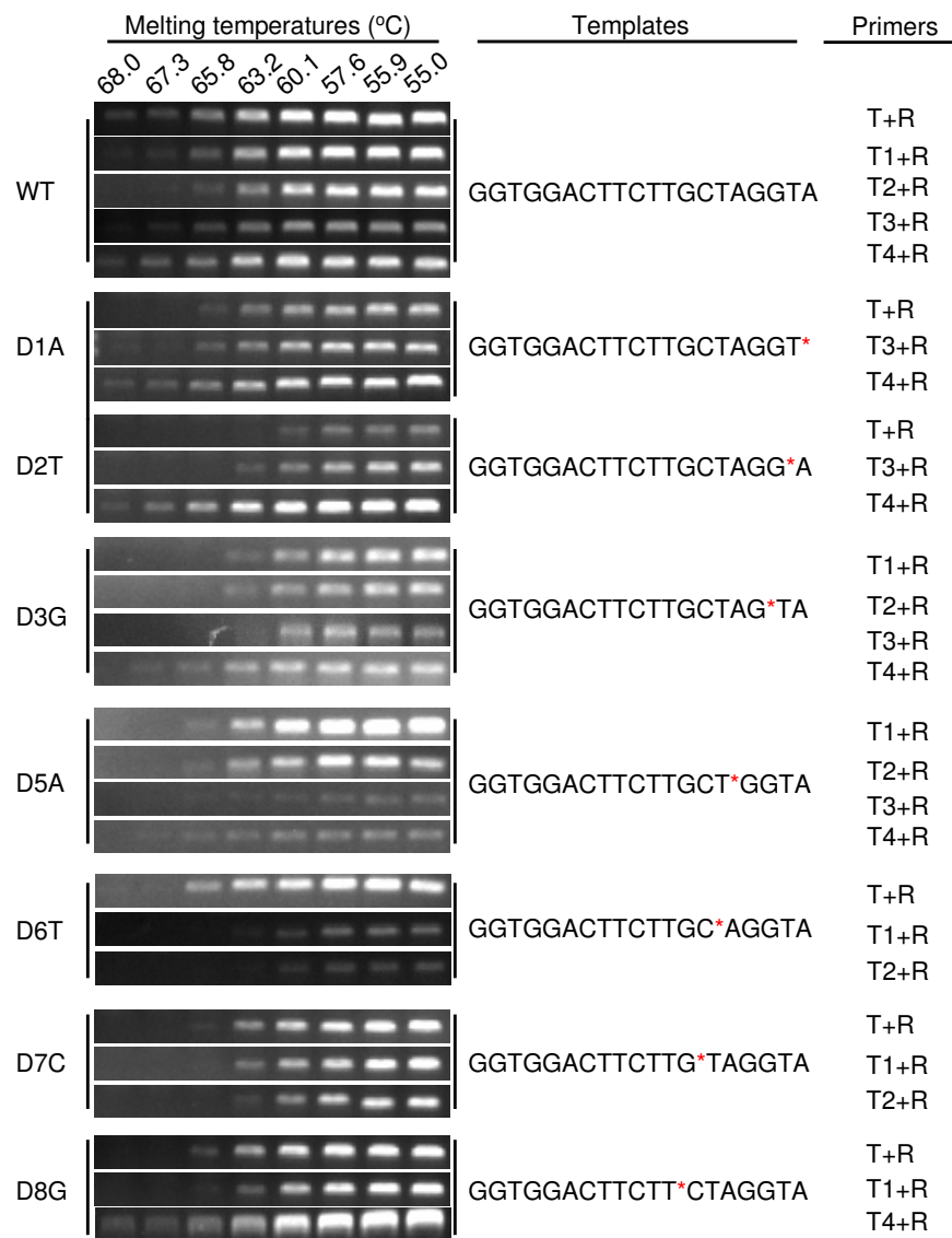
Supplementary Figure 1. The yield of temperature gradient PCR with different single point mutation templates of NiCRTISO (synthesized) and different combination of primers was detected by agarose gel electrophoresis. Equal amount of each templates was added in each PCR system. The red asterisk indicates a lack of a base pair. At least three independent biological replications were amplified to each PCR.
