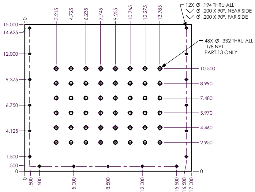
4 DC-P3R2 SCALE: 1:6 MATL: 1/2 ACRYLIC QTY: 1
