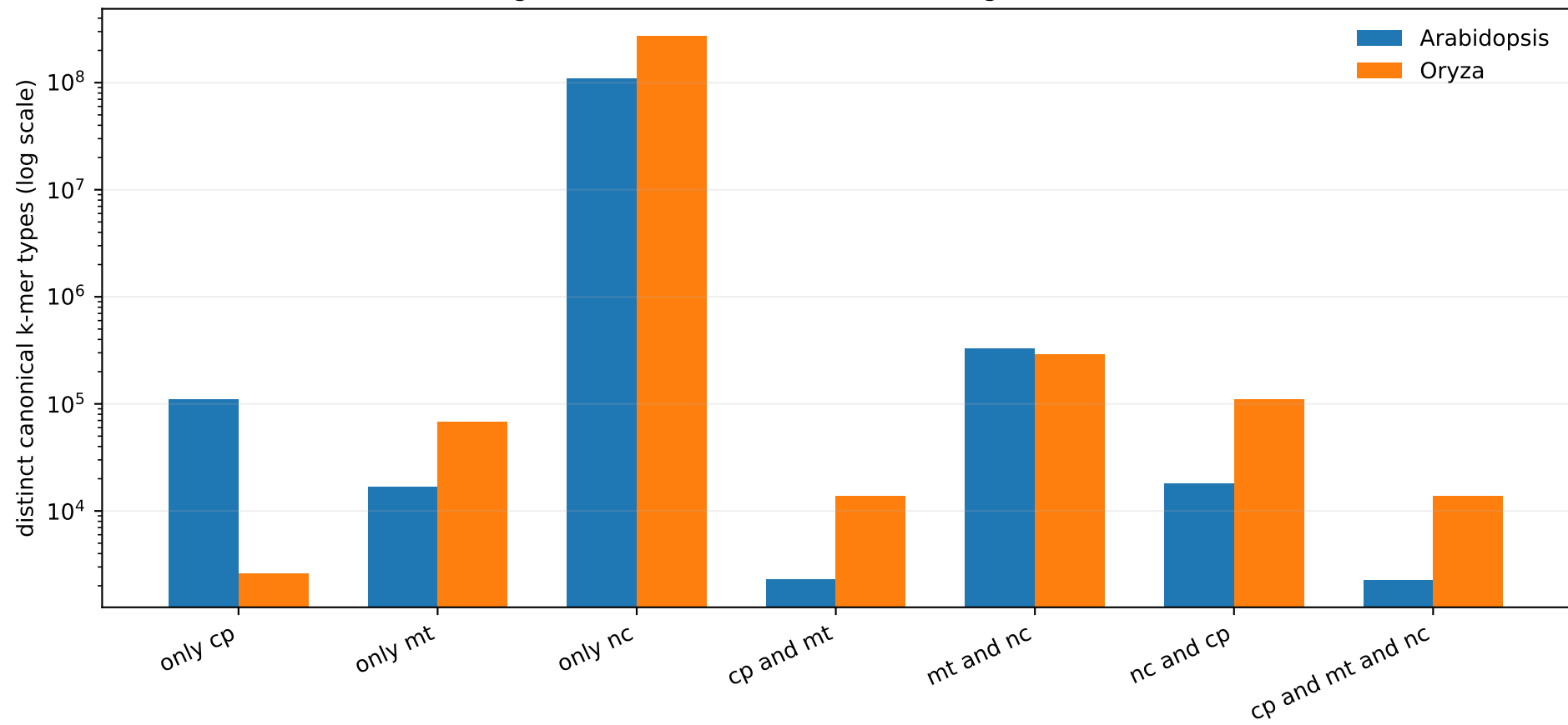
Figure S1. Exclusive and shared categories at k=21
