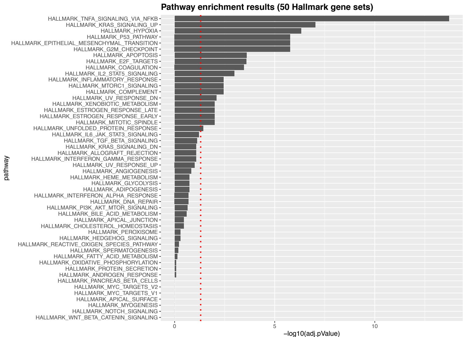
SI Figure 3: Pathway enrichment analysis using the 50 Hallmark gene sets form MSigDB Fischer Exact Test was applied to test for enrichment of Hallmark gene sets within the the 2nd-neighborhood of CLIP2 of the GNA reconstructed from gene set 4. 19 out of 50 gene set exhibited a significant enrichment with an adjusted p-value < 0.05 (red dashed line)
