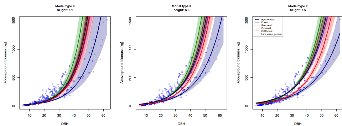
Figure 2. Effect plots of model type II. The points represent the measurement, the bold lines the fitted curve for the land use class specific model and the shaded areas represent the 95% confidence bands. The tree height has been set to the mean (middle row) or the 25- or 75-percentile from the data.
