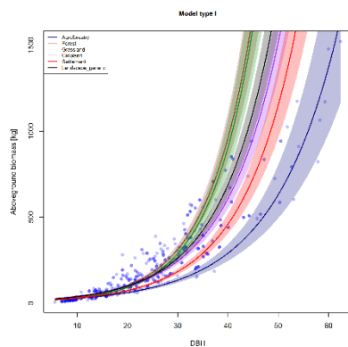
Figure 1. Effect plots of model type I. The points represent the measurement, the bold lines the fitted curve for the land use class specific model and the shaded areas represent the 95% confidence bands.
