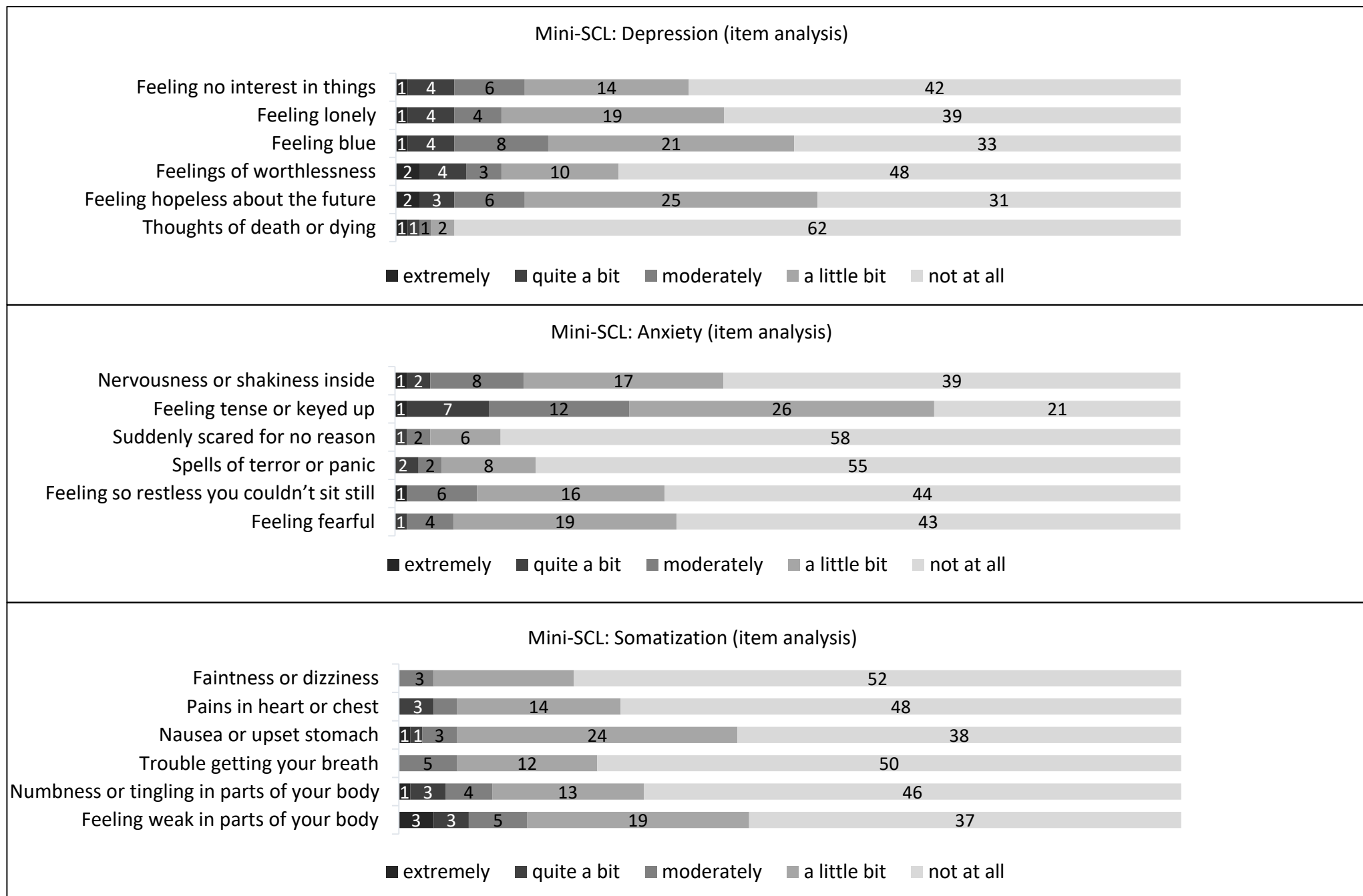
Figure 3: Item analysis of Mini-SCL scales ,Depression', ,Anxiety' and ,Somatization' in caregivers (self-report)
