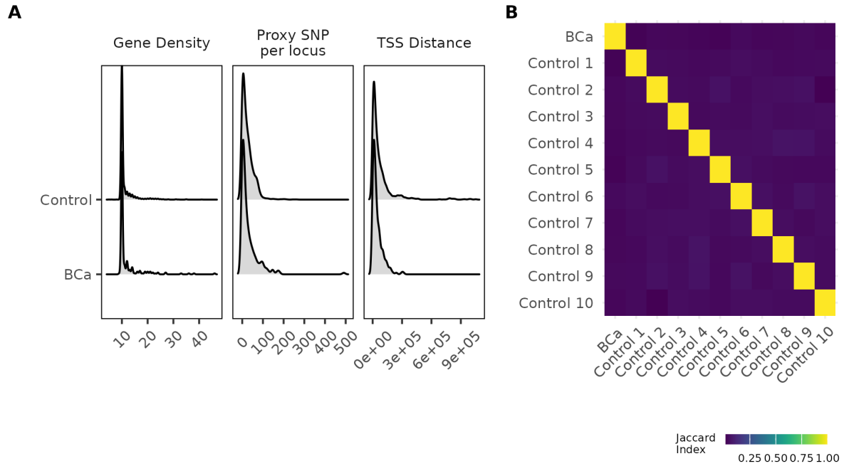
Supplemental Figure 2: Curation of control set. (A) Distribution of gene density, proxy SNP per locus, and distance from transcription start site for BCa and control SNPs. (B) Jaccard index heatmap comparing candidate gene sets in BCa and all control sets.
