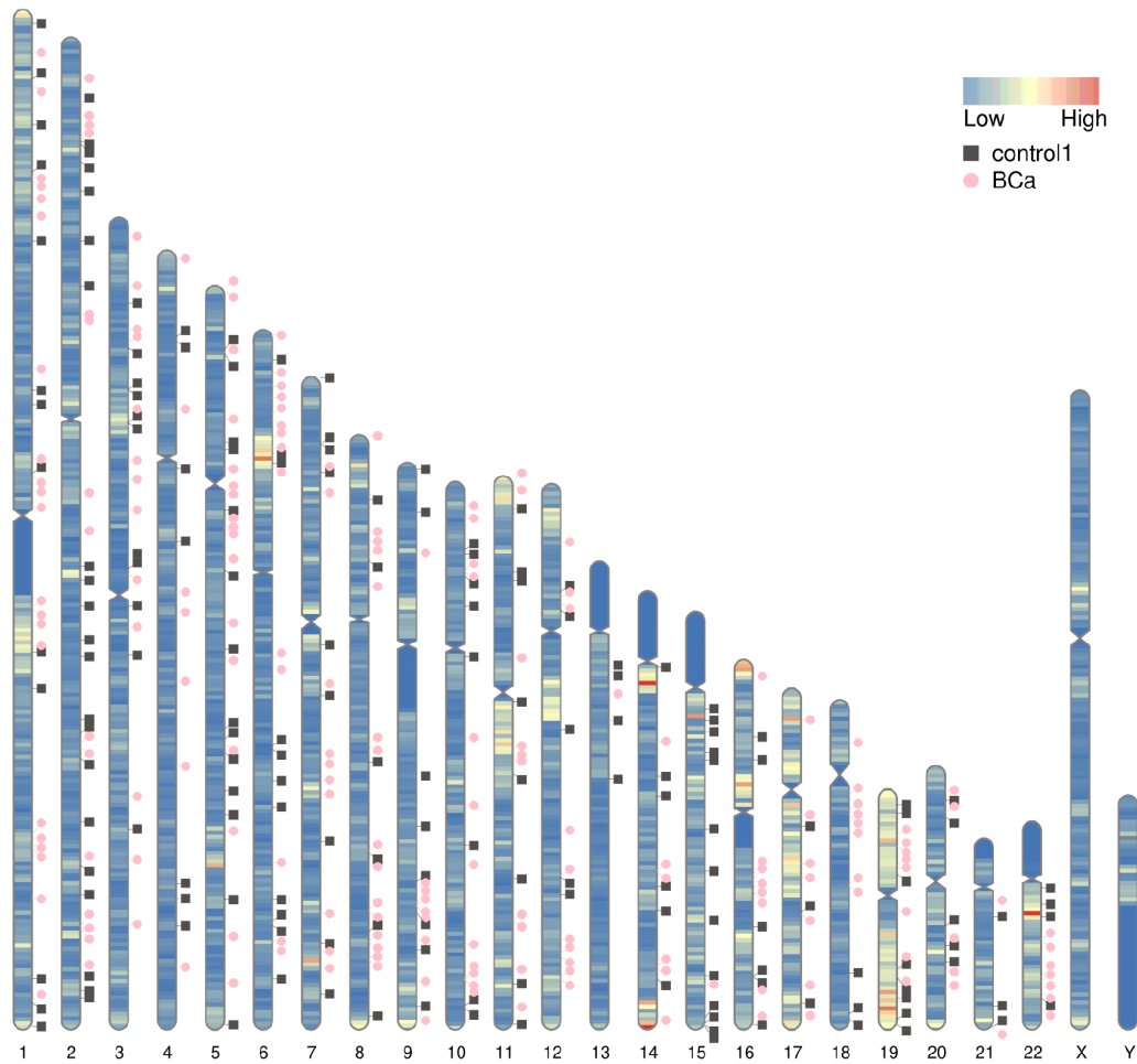
Supplemental Figure 1: Idiogram of BCa and control 1. Chromosome mapping represents gene density. The remaining nine controls are not shown.
