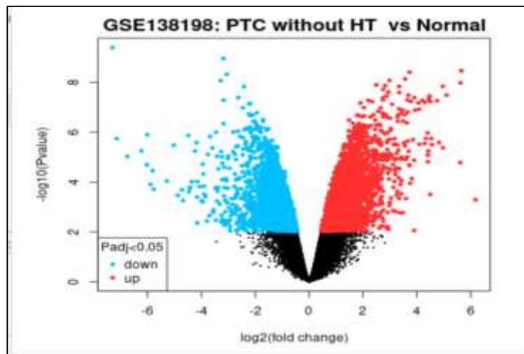
a Volcano plot of differentially expressed genes
