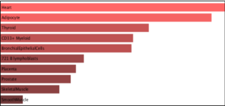
g. Cell type- Human gene Atlas
