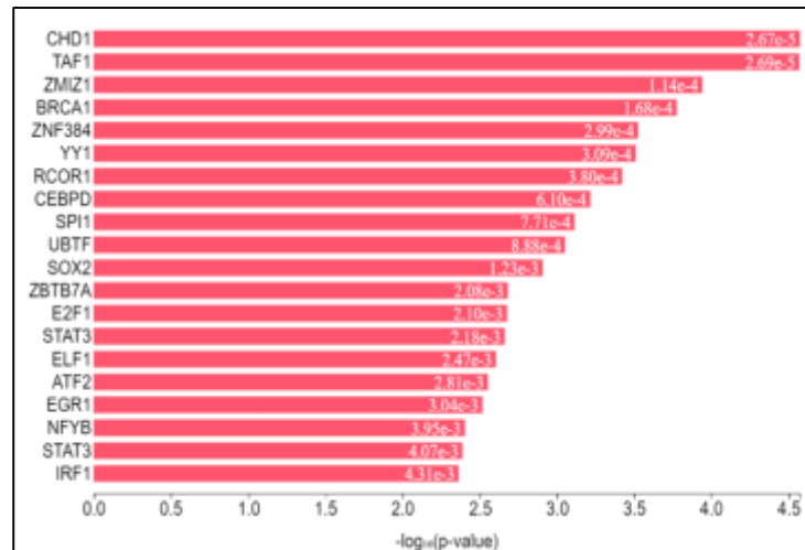
b Transcription Factor Enrichment Analysis (TFEA)
