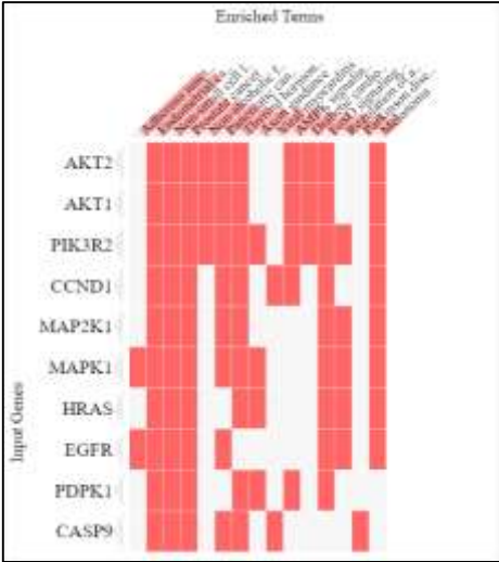
d. GO Molecular Function
