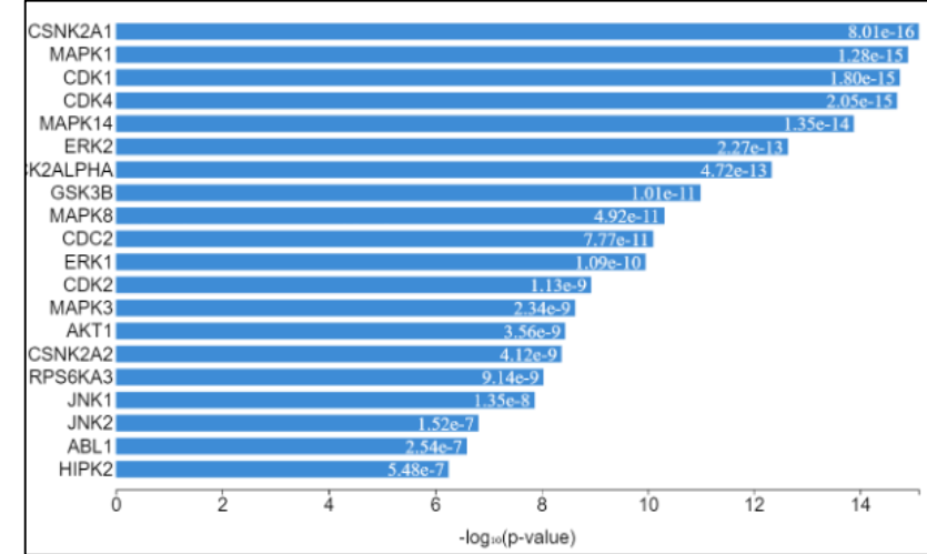
c Kinase Enrichment Analysis (KEA)
