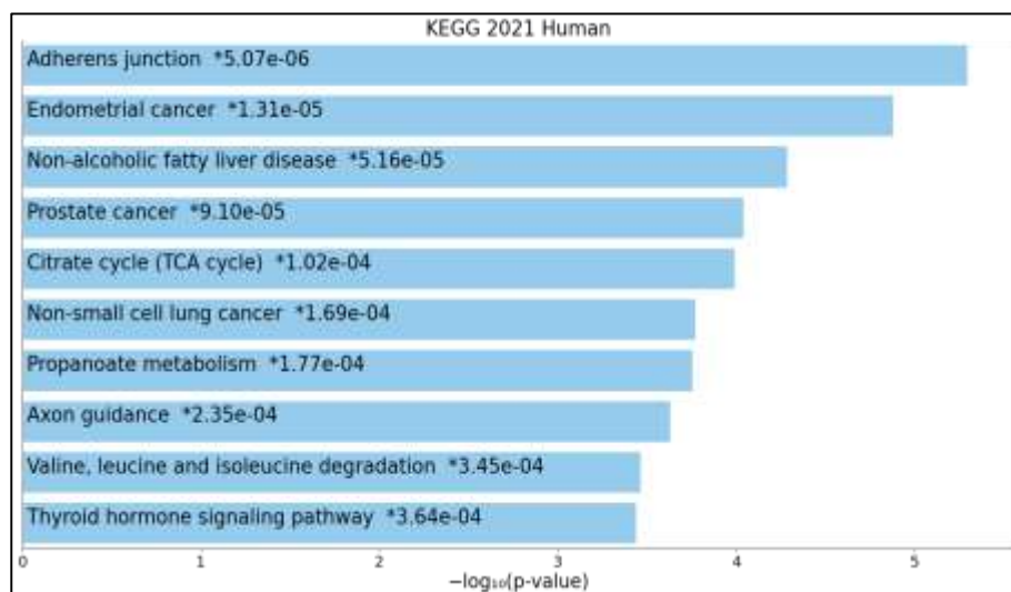
d Enrichment analysis: KEGG pathway
