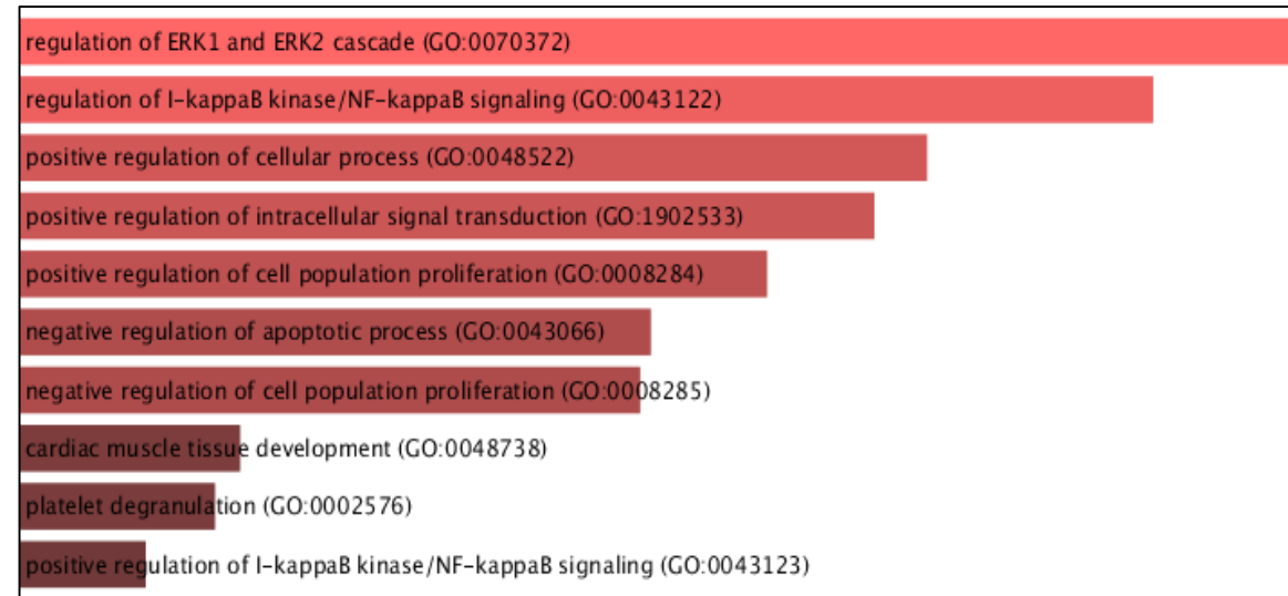
e GO Biological Process
