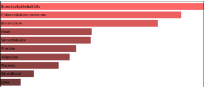
g. Cell type- Human gene Atlas
