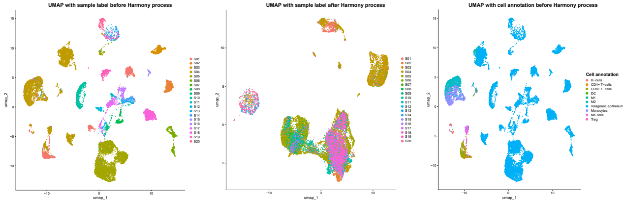
Supplementary Figure 1. Harmony integration reduces inter-sample batch effects.
