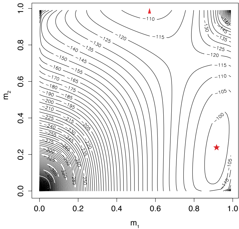
Contour plot of log likelihood function
