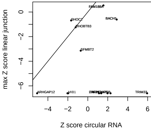
Adrenal junctions circular vs. max linear z score per gene Fetal_Adrenal_360
