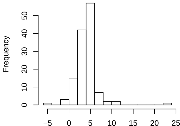
All circular z scores Heart
