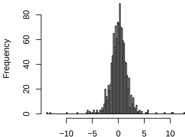
All linear junction z scores Adrenal
