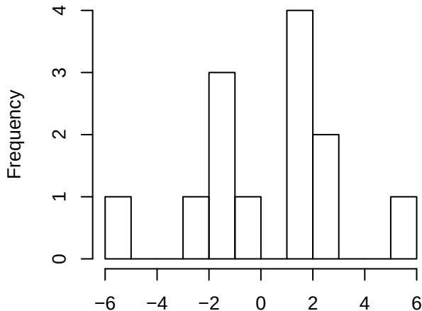
All circular z scores Adrenal
