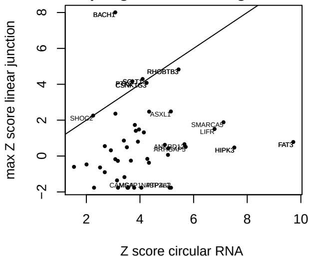
Lung junctions circular vs. max linear z score per gene Fetal_Lung_361
