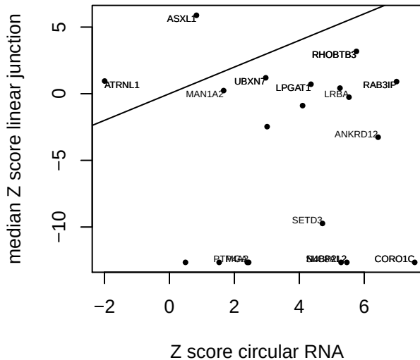
Intestine junctions circular vs. median linear z score per gene Fetal_Intestine_360
