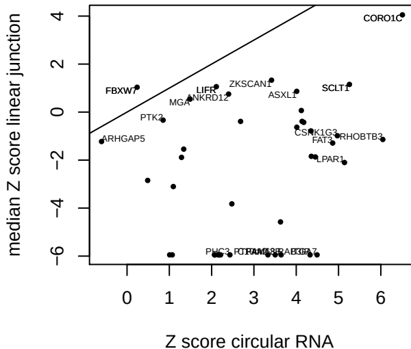
Stomach junctions circular vs. median linear z score per gene Fetal_Stomach_360
