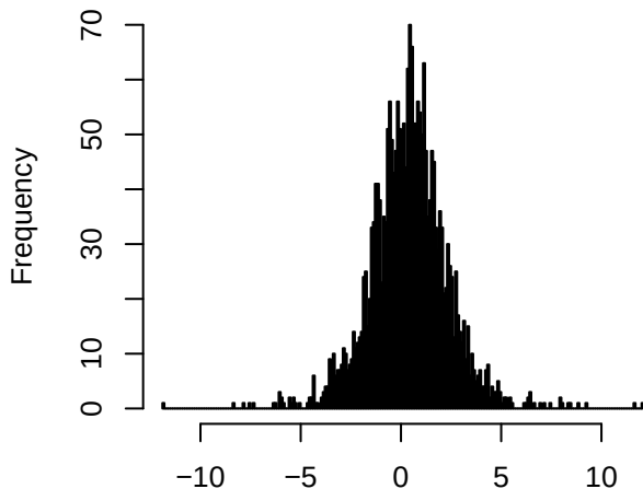
All linear junction z scores Lung
