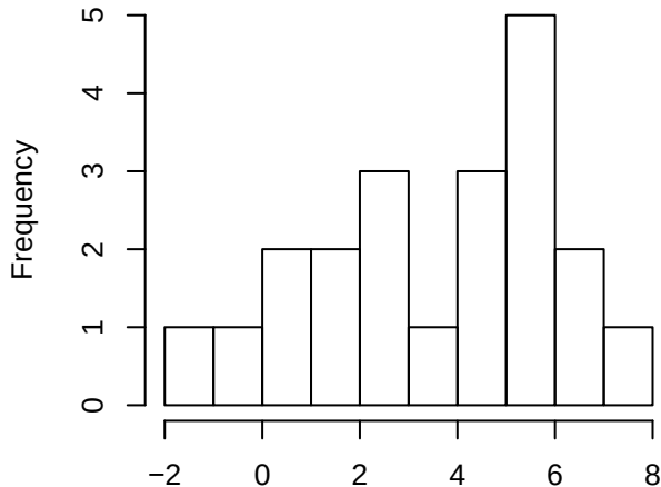
All circular z scores Intestine
