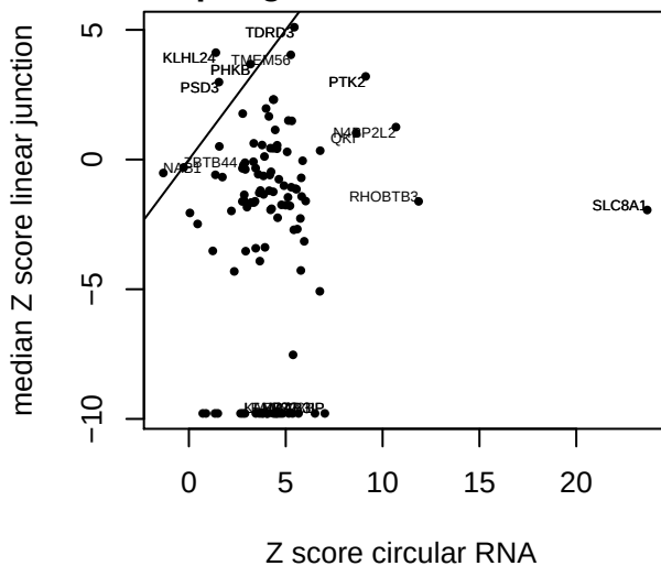
Heart junctions circular vs. median linear z score per gene Fetal_Heart_361
