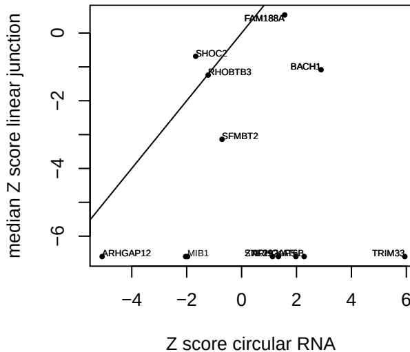
Adrenal junctions circular vs. median linear z score per gene Fetal_Adrenal_360
