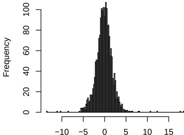
All linear junction z scores Stomach
