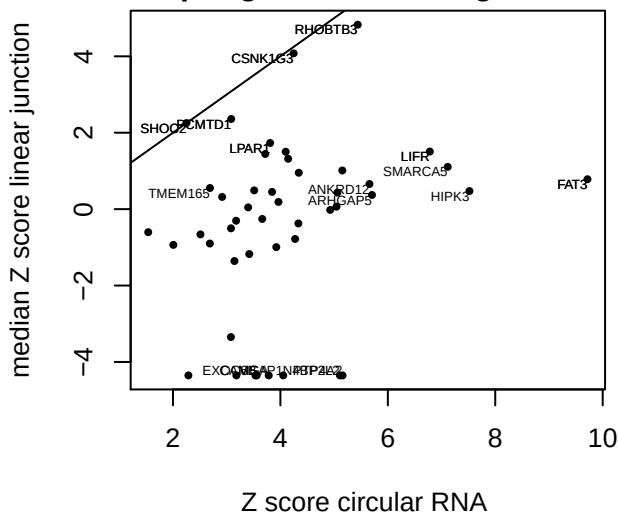
Lung junctions circular vs. median linear z score per gene Fetal_Lung_361
