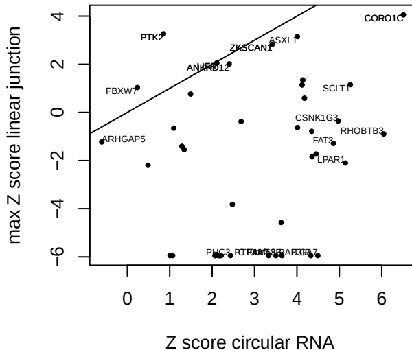
Stomach junctions circular vs. max linear z score per gene Fetal_Stomach_360
