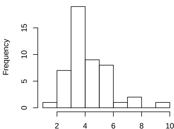
All circular z scores Lung
