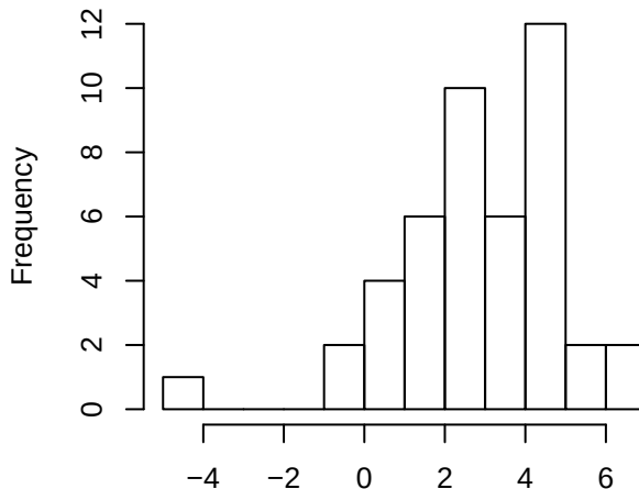
All circular junction z scores Stomach
