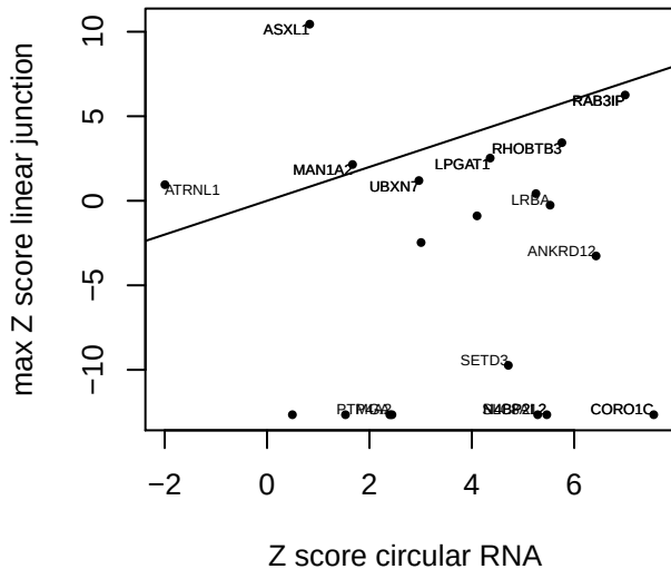
Intestine junctions circular vs. max linear z score per gene Fetal_Intestine_360
