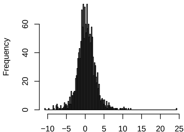
All linear junction z scores Intestine
