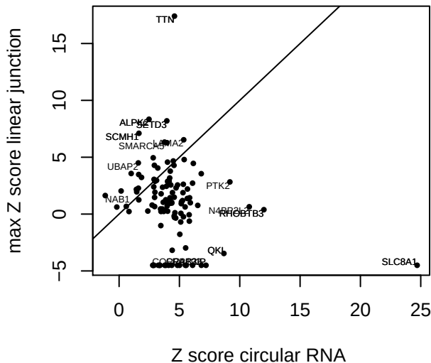
Heart junctions circular vs. max linear z score per gene Fetal_Heart_361
