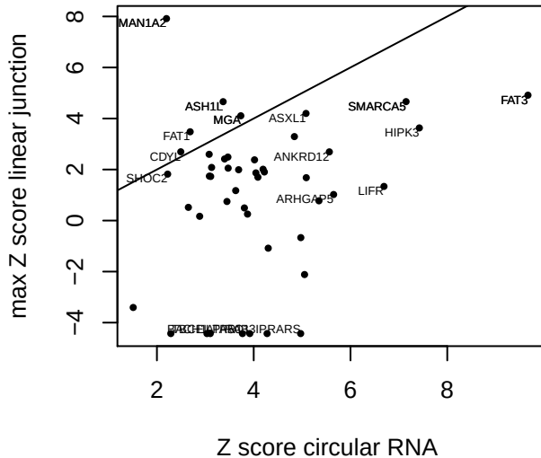
Lung junctions circular vs. max linear z score per gene Fetal_Lung_361
