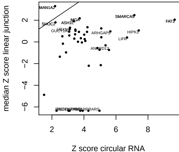
Lung junctions circular vs. median linear z score per gene Fetal_Lung_361
