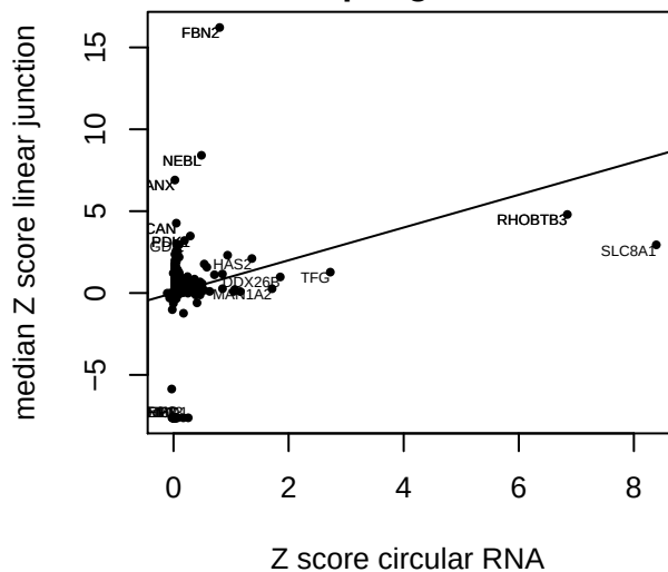
junctions circular vs. median linear z score per gene
