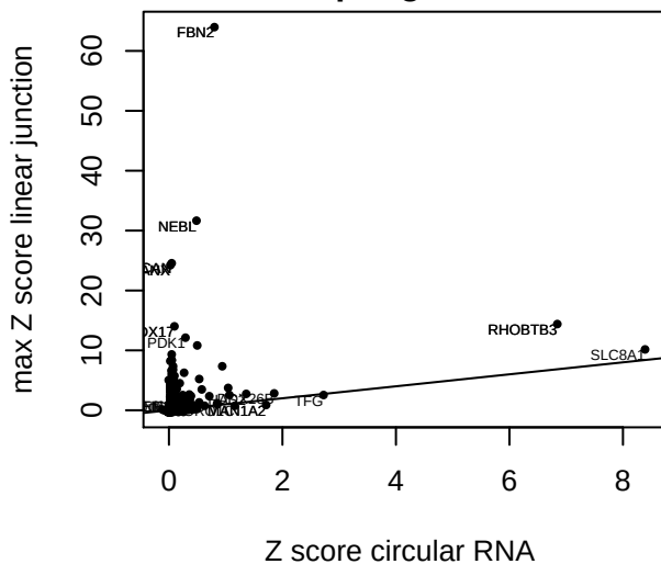
junctions circular vs. max linear z score per gene
