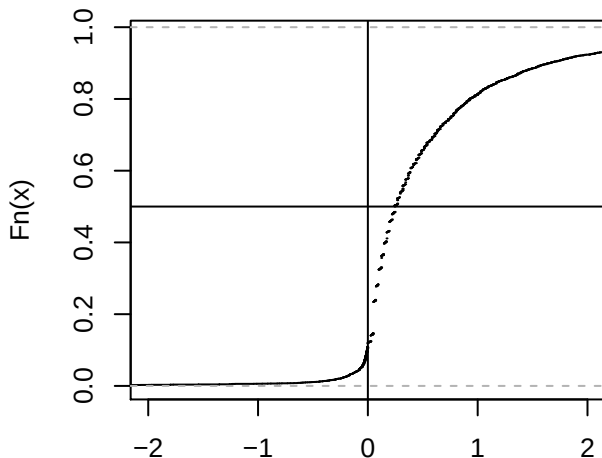
All linear junction z scores
