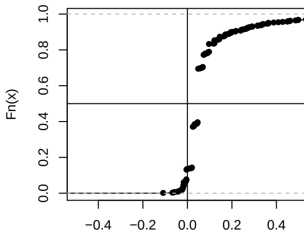
All circular z scores
