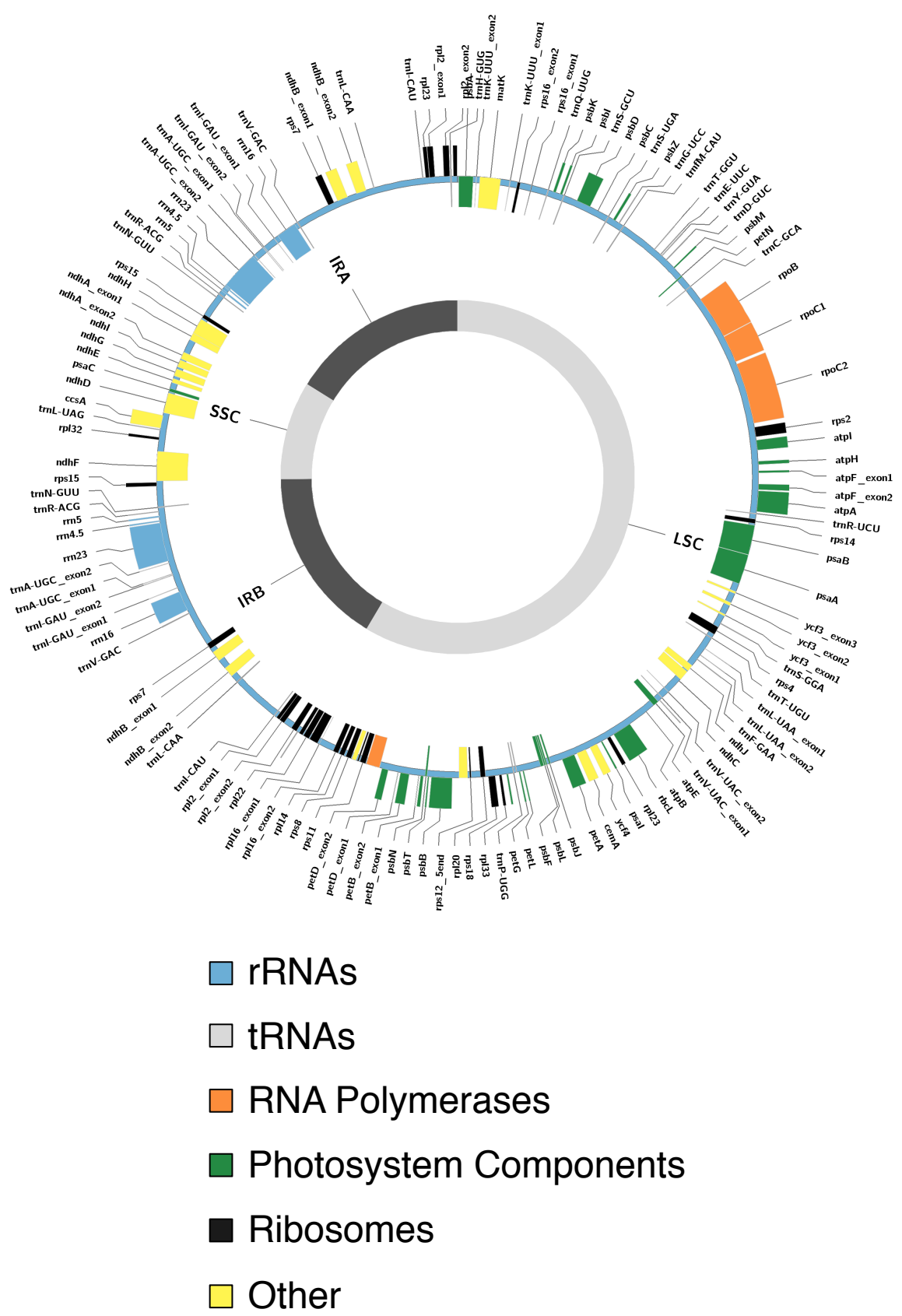
Figure S1: Chloroplast genome annotation.
