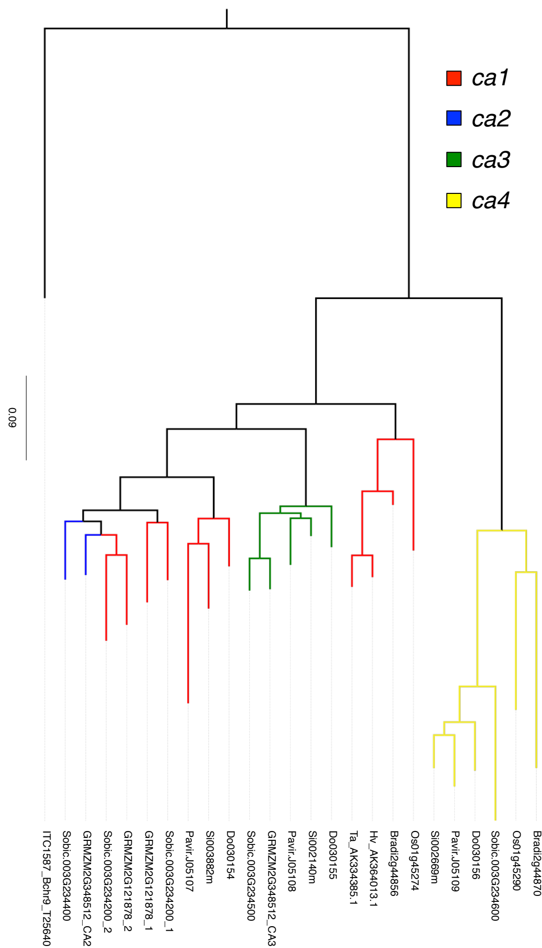
Figure S4: Carbonic anhydrase gene tree.
