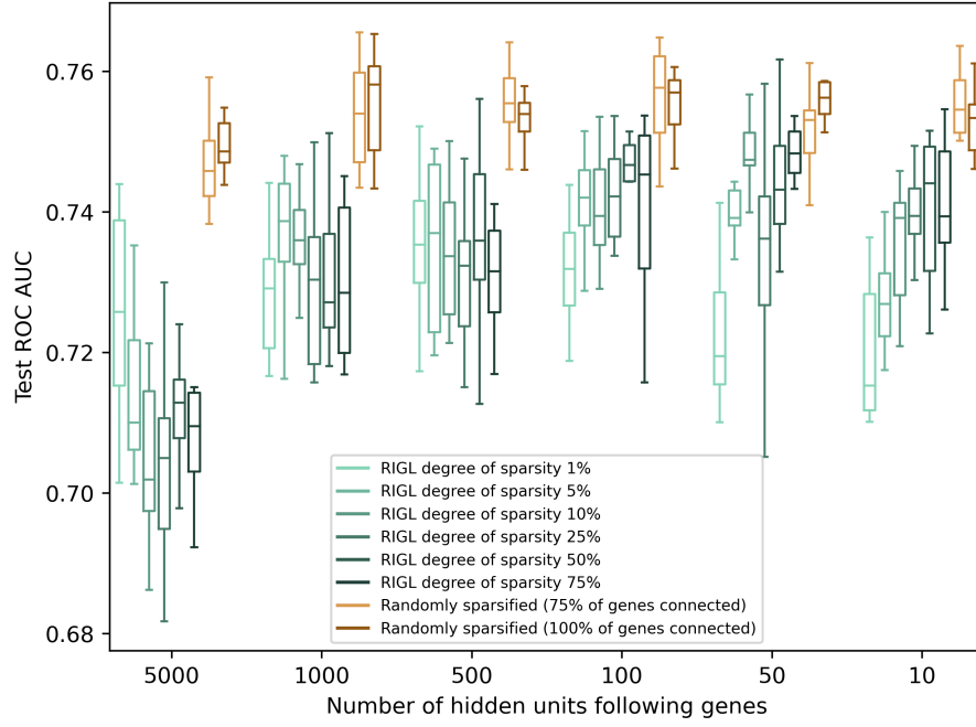
Figure 1: Benchmarking of different degrees of sparsity and hidden units for the Rigl method and the randomly sparsified model.
