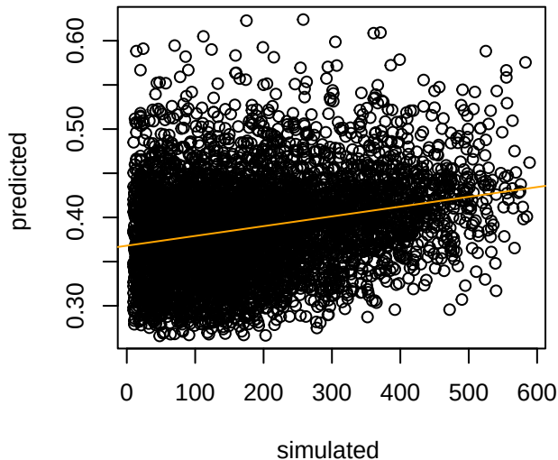
tAdmxEU_NAa Correlation = 0.269
