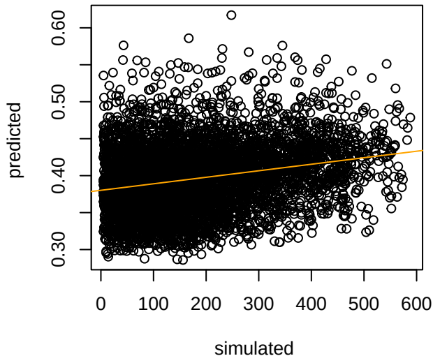
tAdmxWaf_Arab Correlation = 0.273
