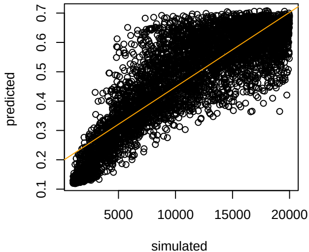
NeNAfb Correlation = 0.853
