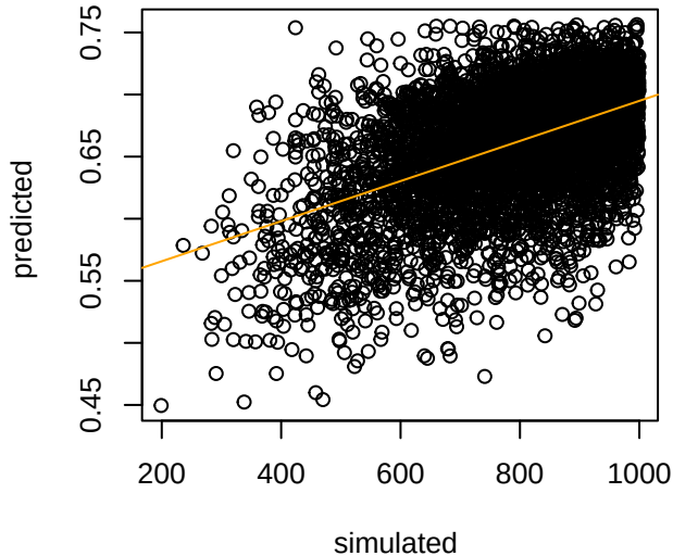
tNAfb_NAfa_ME_EU Correlation = 0.516
