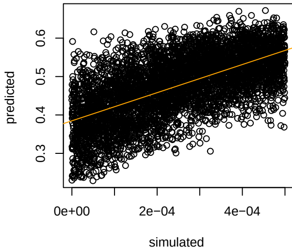
migrationEAf_to_WAf
