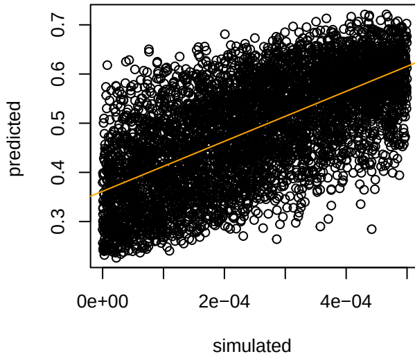
migrationKhs_to_EAf
