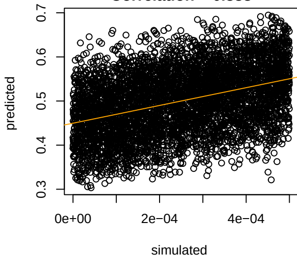
migrationWaf_NAfa
