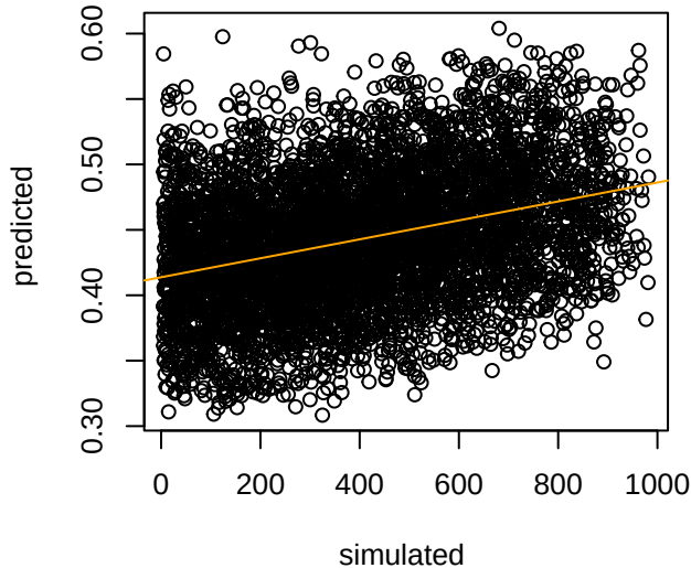
tAdmxWaf_Amazigh
