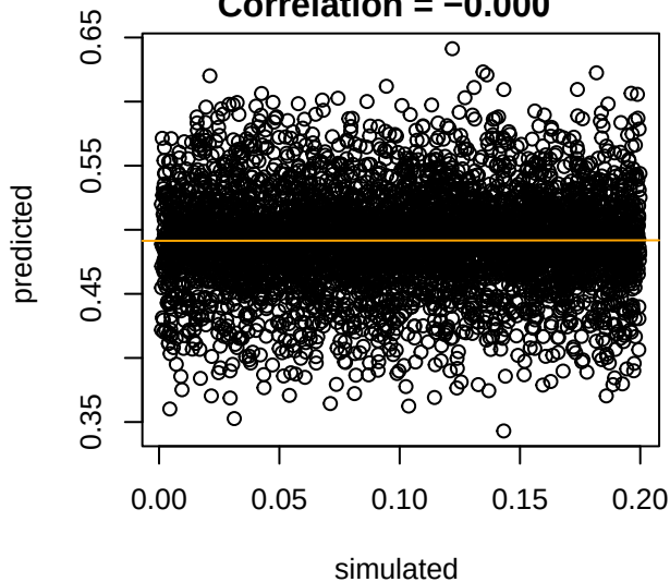
admixtureBEi_AMENAU
