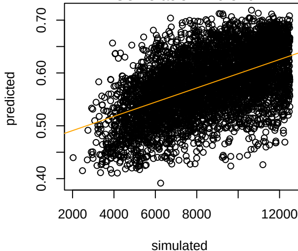
tNAfb_NAfa_ME_EU_BEi_EAs_ Waf_Khs_Xa
