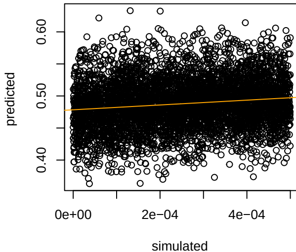
migrationME_NAfb Correlation = 0.149
