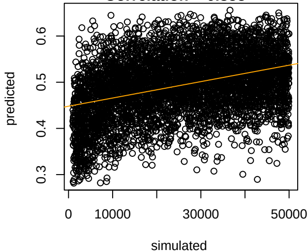
NeNAfb_NAfa_ME_EU_BEi_EAs_Waf_ Khs_Xa
