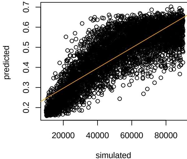
NeWAf Correlation = 0.848
