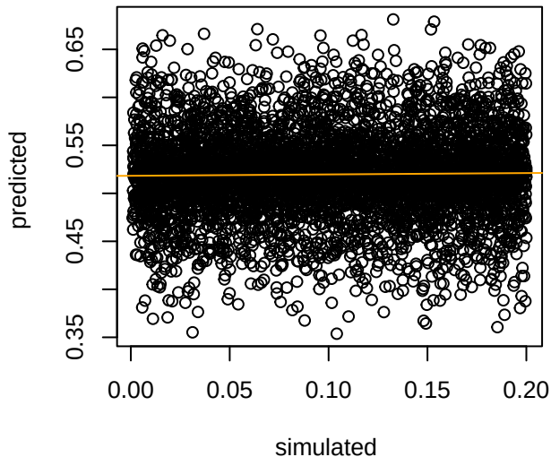
admixtureME_NAa Correlation = 0.009
