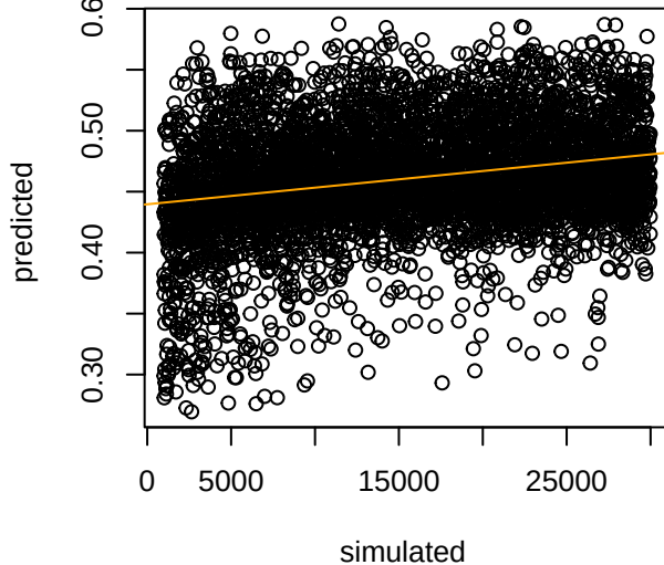
NeNAfa_ME Correlation = 0.247
