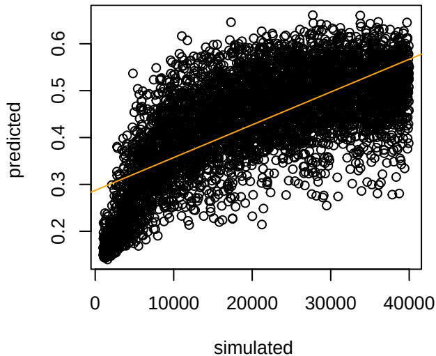
NeAfa Correlation = 0.700
