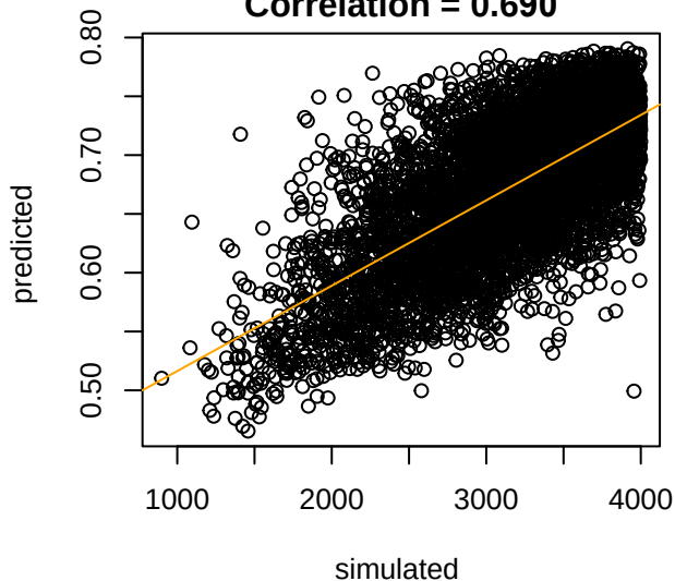
tNAfb_NAfa_ME_EU_EAs_EAf
