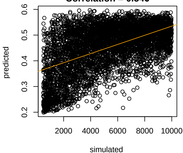
NeNAfb_NAfa_ME_EU_BEi_EAs
