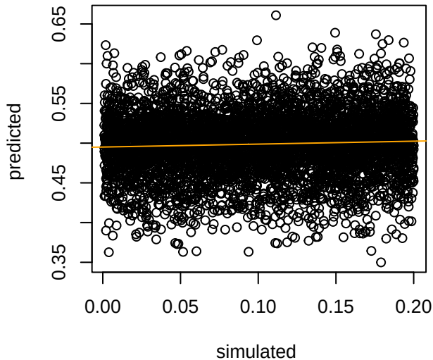
admixtureBEi_MENAU Correlation = 0.026
