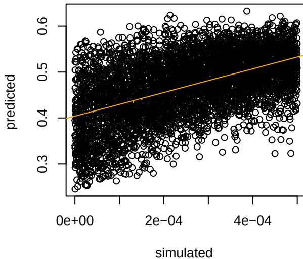
migrationWAf_to_EAf
