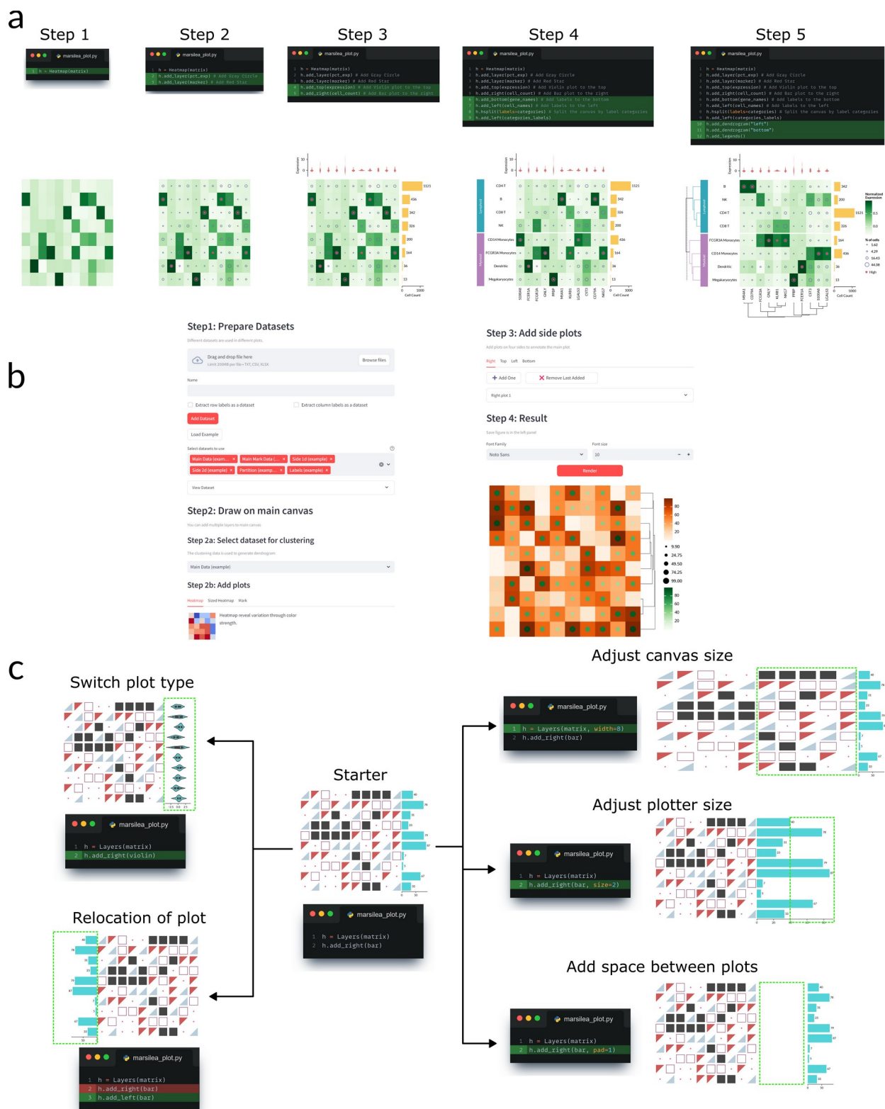
Fig. S2: Demonstration of the a) programmatic and b) web-based interfaces of Marsilea. c) Demonstration of the simplicity of making layout adjustments in Marsilea.
