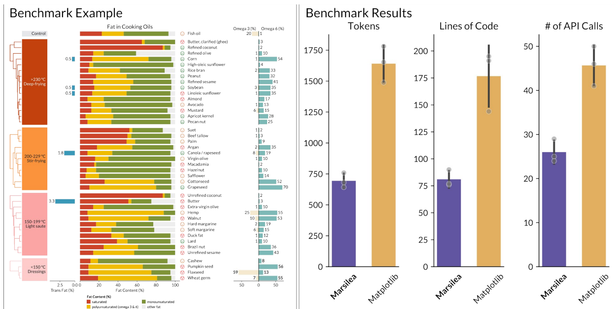
Fig. S3: The plot we used for benchmarking and the benchmark results.
