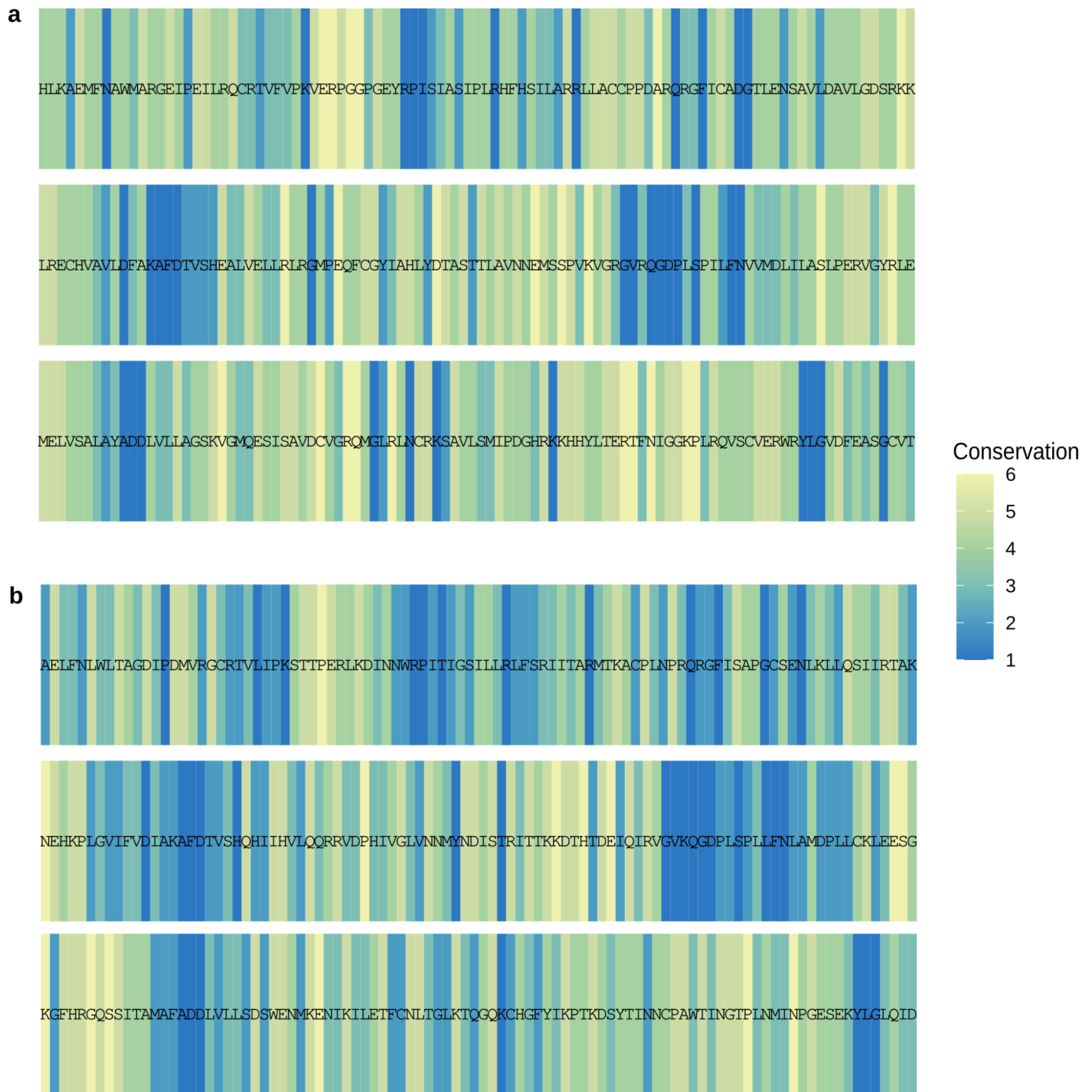
Figure S11: Site-specific conservation of individual residues in lineage D and A R2s superimposed with RT residues from (a) B. mori (lineage D) and (b) Z. albicollis (lineage A, reconstructed from short-reads). Conservation is shown as high (1-3) to low (4-6).
