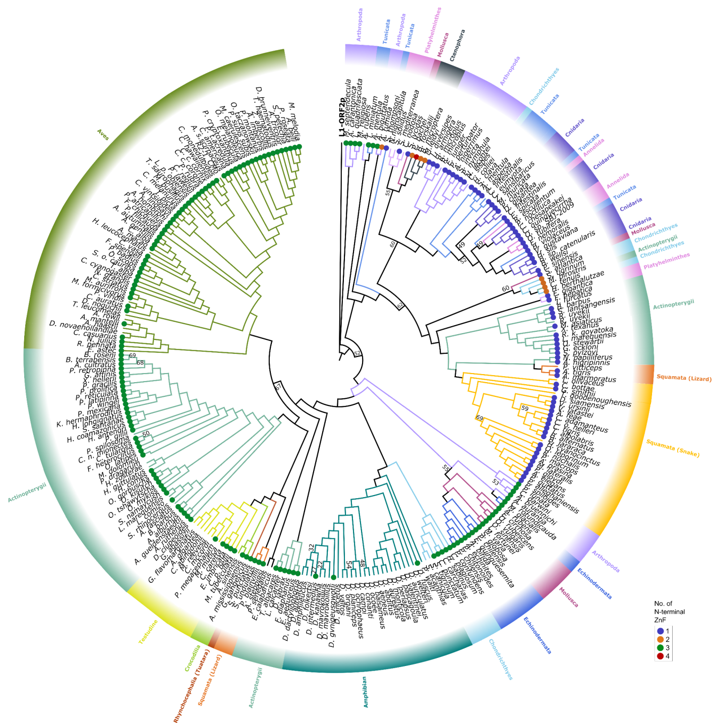
Figure S4.1: Topology only (branch length ignored) phylogenetic tree of all site-specific R2s with a protein coding region rooted with human L1 (MFP model finder, 1000 bootstraps, support values under 70 shown). Coloured circles indicate the number of N-terminal zinc fingers. R2s without a coloured circle indicate the element has a partial ORF.
