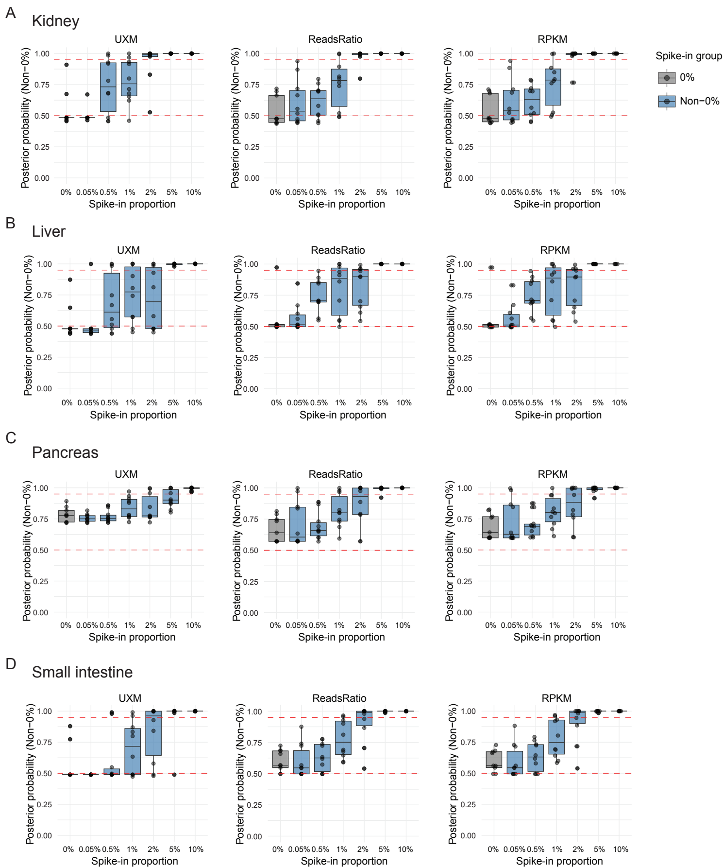
Fig S5. Posterior probability by naive Bayes inference for target cell type.
