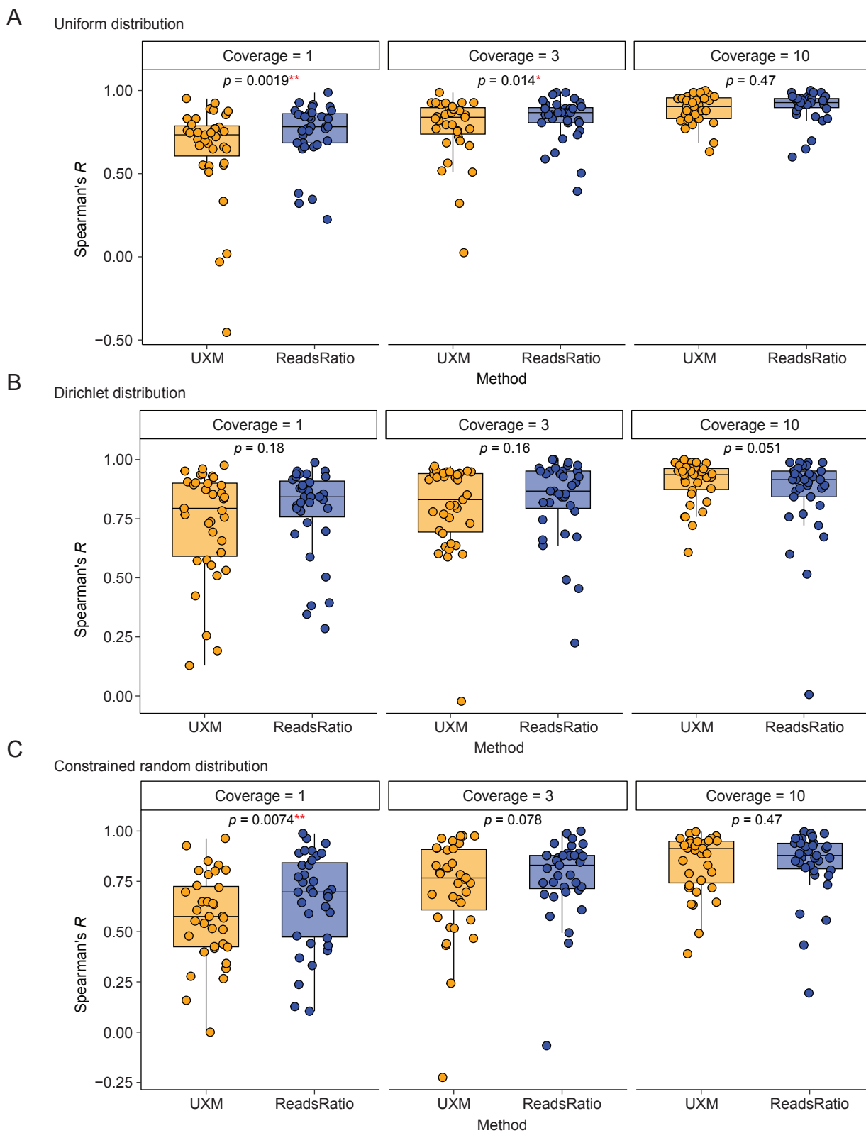
Fig S8. Comparison of deconvolution results between UXM and ReadsRatio on simulated data with known ground truth proportion for each cell type.
