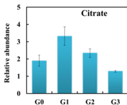
Figure S1 Variations of citrate during the adaptation process to multiple inhibitors. The relative abundance was calculated by normalizing the peak area of citrate with internal standard (IS) in the same chromatogram. Results are expressed as mean \pm standard error of the mean ( n>5 ).
