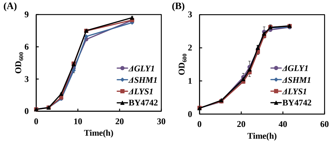
Figure S2 The growth behaviors of the strain BY4742, \Delta GLY1 , \Delta SHM1 and \Delta LYS1 . (a) The strains were cultivated in YPD medium in the absence of multiple inhibitors. (b) The strains were cultivated in YPD medium in the presence of 1.0 g/L furfural, 4.0 g/L acetic acid and 0.4 g/L phenol. Results are the mean of duplicate experiments and error bars indicate s.d.
