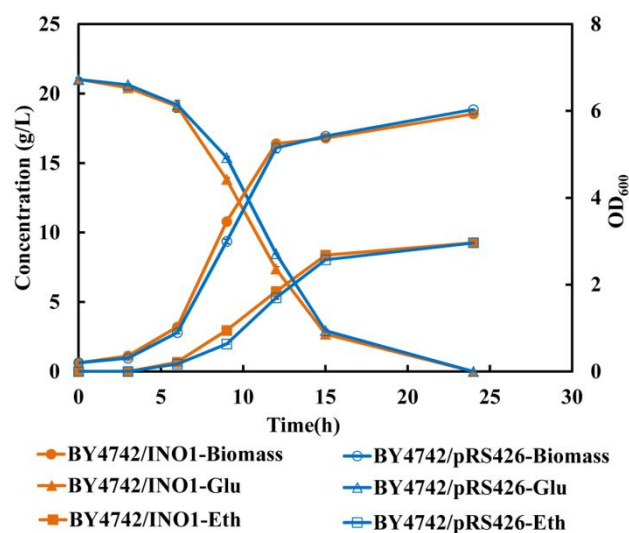
Figure S7 The growth profiles, glucose consumption and ethanol production of the recombinant strain BY4742/INO1 and its control strain BY4742/pRS426 in SC-Ura medium in the absence of multiple inhibitors. Results are the mean of duplicate experiments and error bars indicate s.d.
