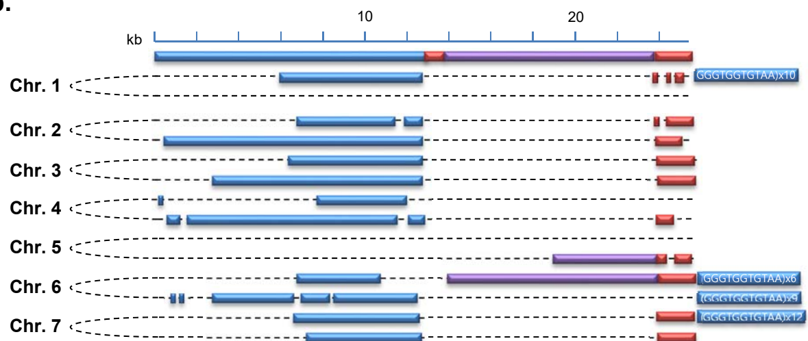
Figure S11. Identification of putative centromeres (a) and telomere regions (b) of S. fibuligera ATCC 36309 chromosomes.
