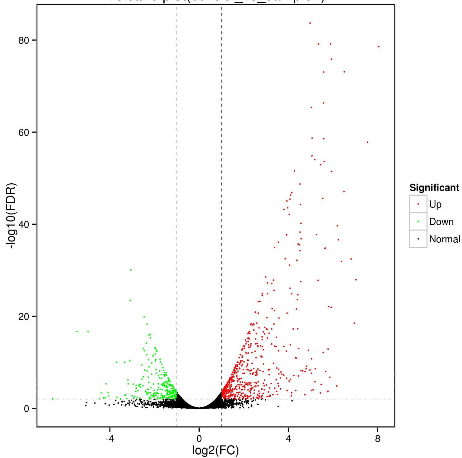
Volcano plot(control_vs_sample1)
