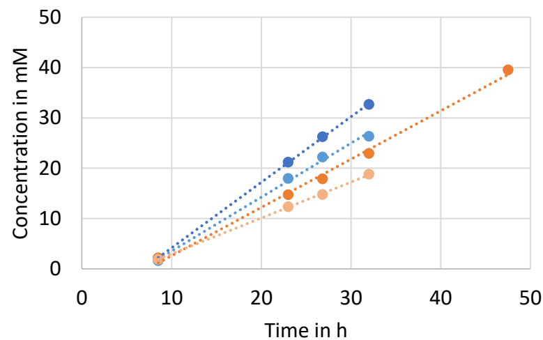
Ethyl acetate
