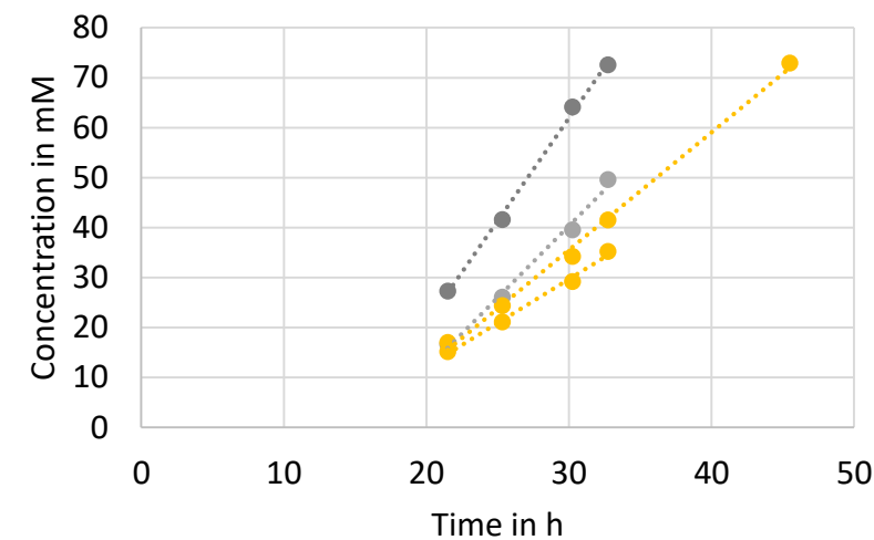
Hydrogen
