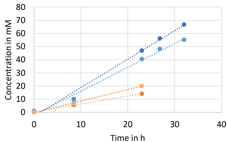
Formate
