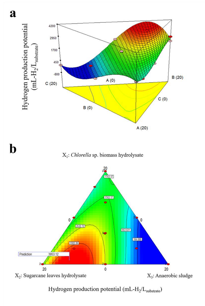
Fig. S1 The mixture design plots for hydrogen production potential from the co-digestion process.
