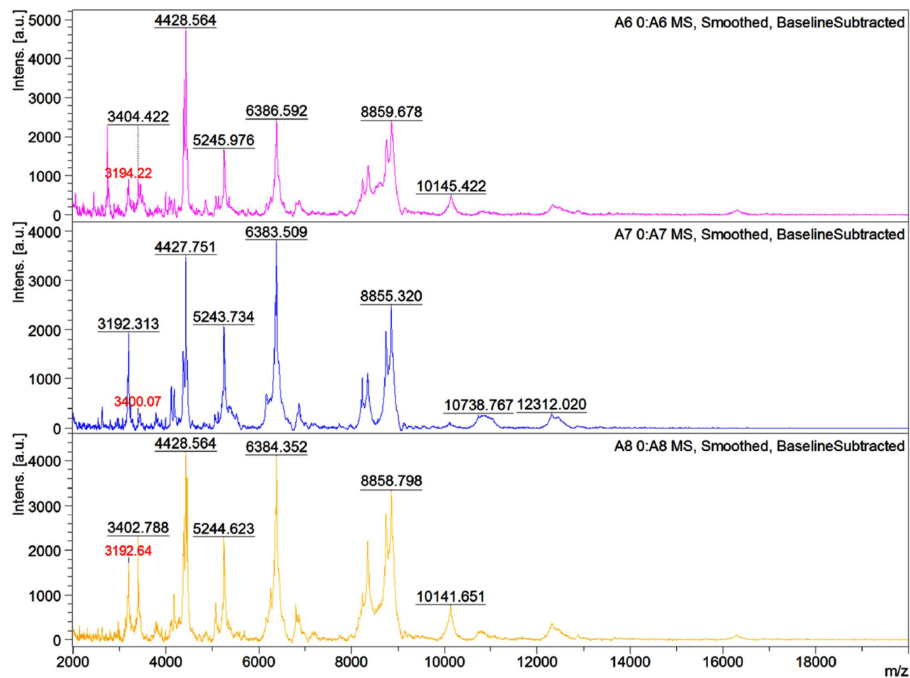
Figure S2. MALDI-TOF MS spectra of three representative specimens of An. culicifacies .
