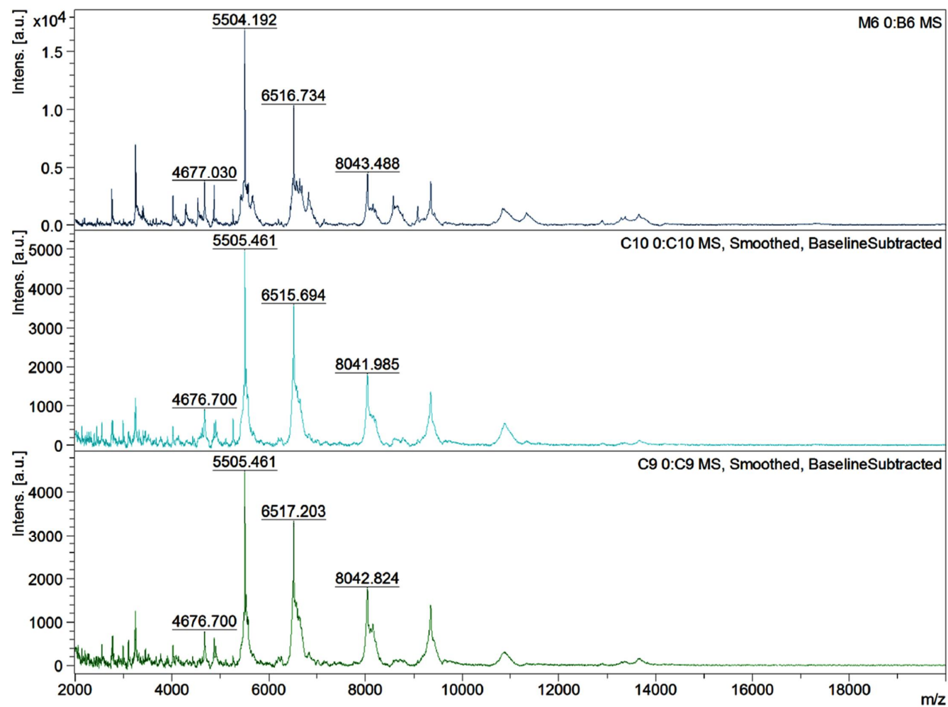
Figure S5. MALDI-TOF MS spectra of three representative specimens of Ae. albopictus .
