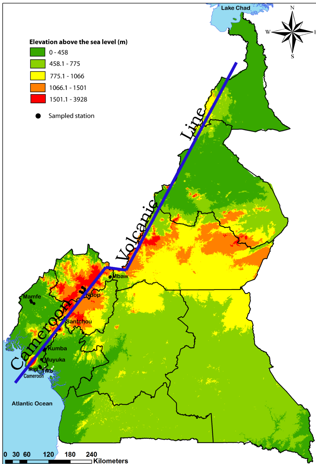
Additional file 1: Figure S1. Cameroon volcanic line.
