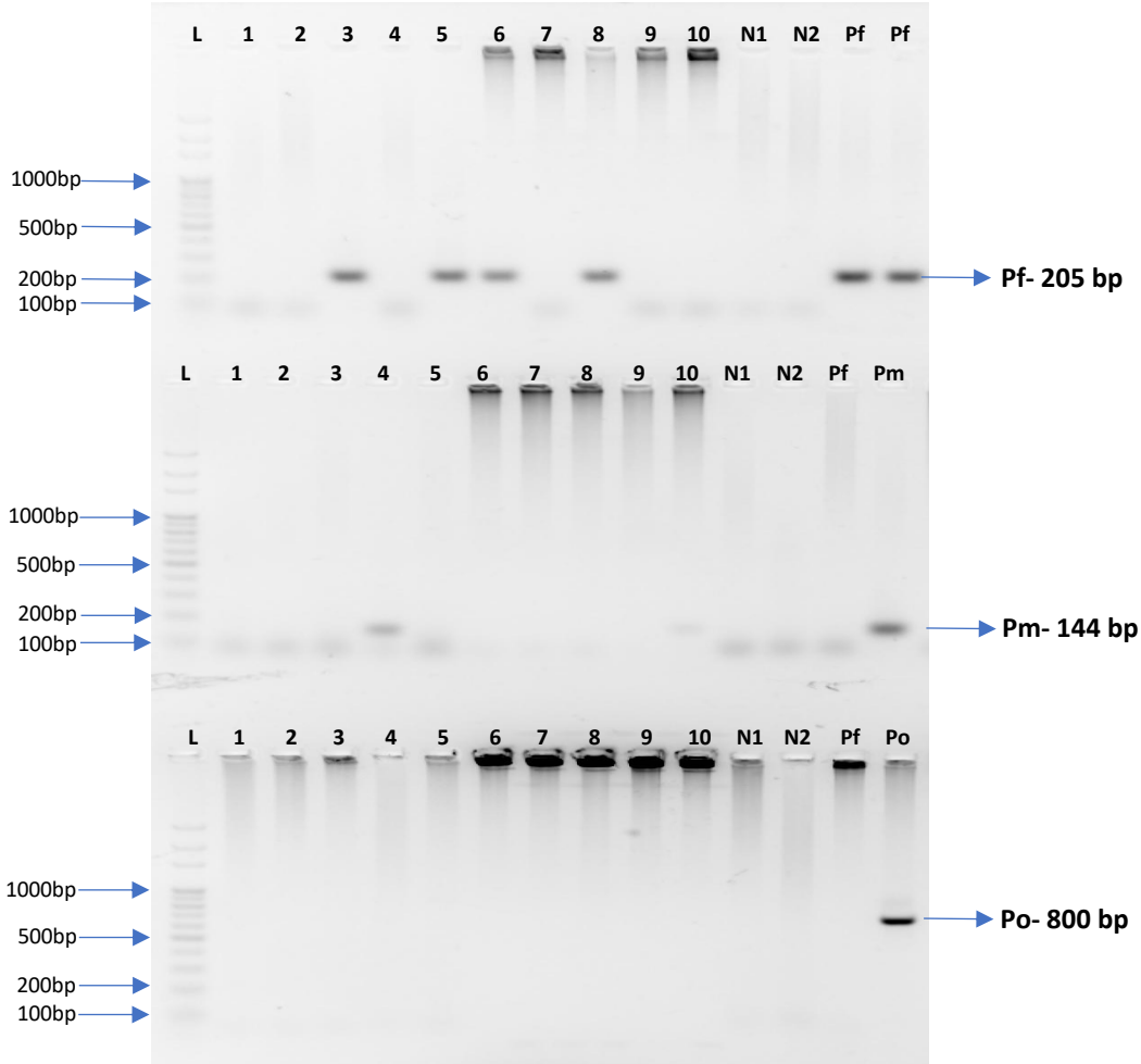
2% Agarose Gel
