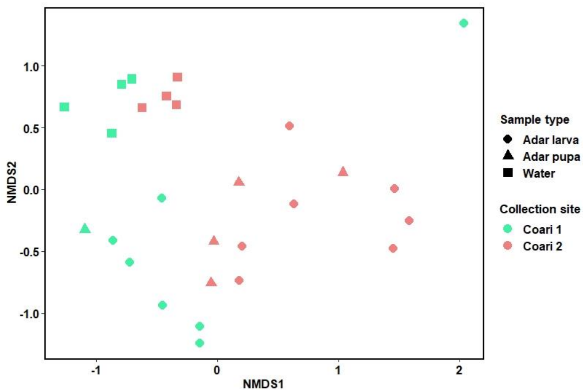
Fig. S4. Non-metric multidimensional scaling (NMDS) based on Bray-Curtis distances.
