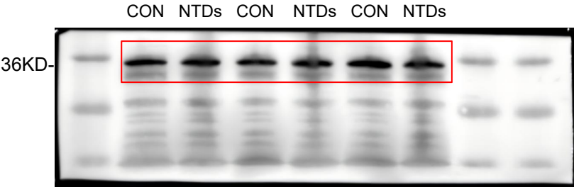
GAPDH
