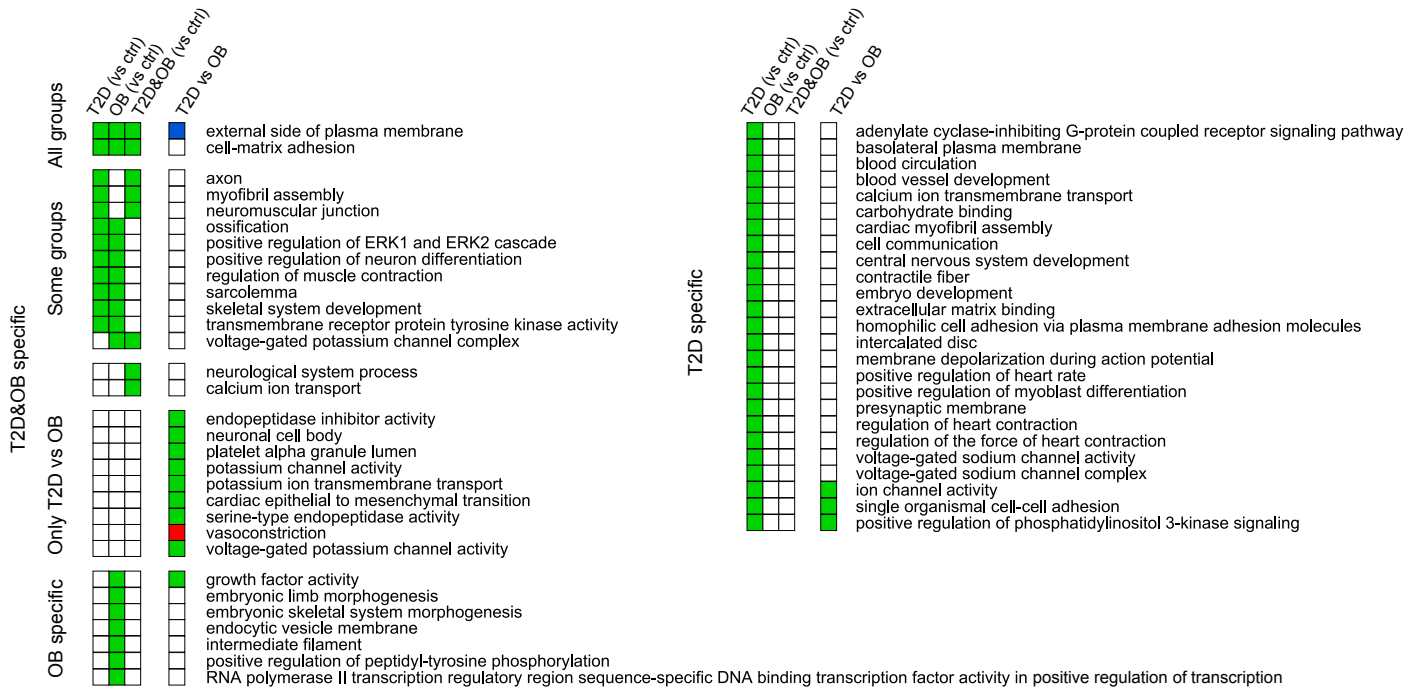
Figure S6. Heatmaps showing significant GO-term gene-sets. Significant gene-sets are marked as either red (up-regulated), blue (down-regulated), or green (unspecifically regulated).
